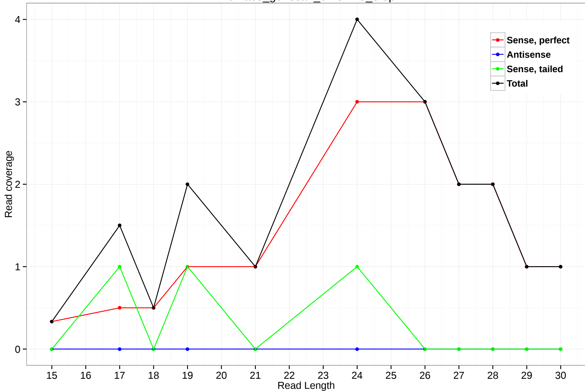
rheMac3_genscan_chr3.119_3.3p
