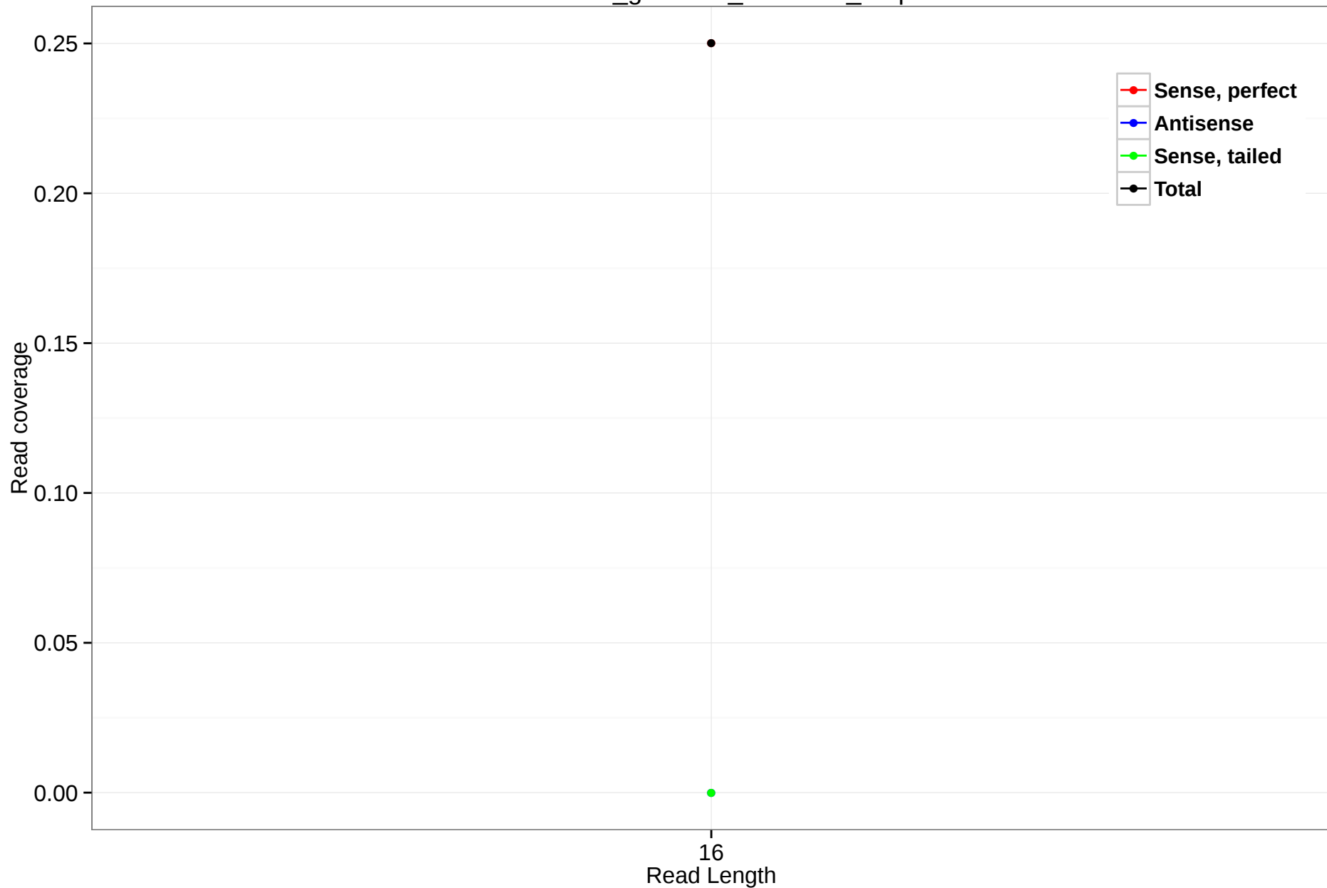
rheMac3_genscan_chr3.117_3.3p
