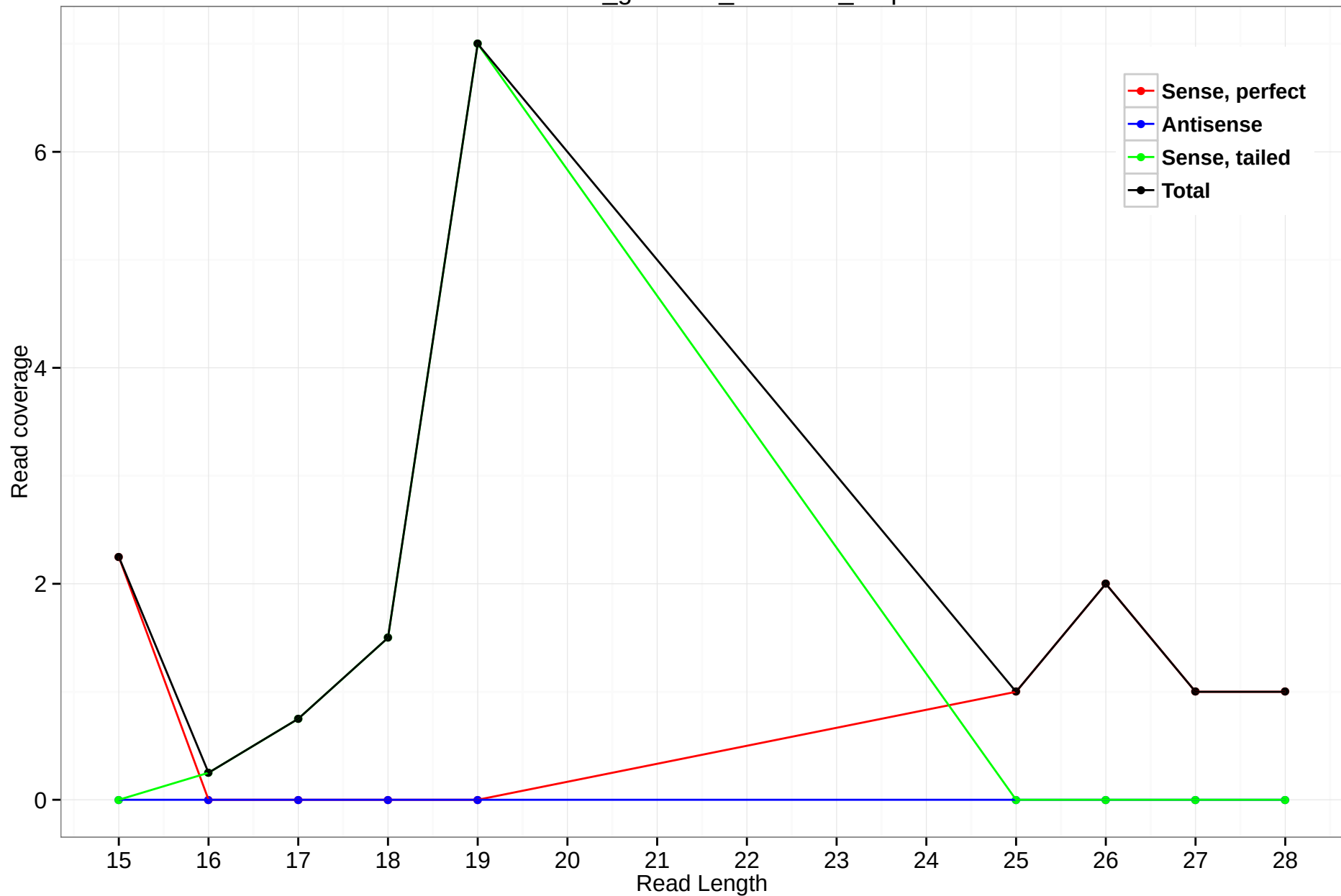
rheMac3_genscan_chr3.079_9.5p
