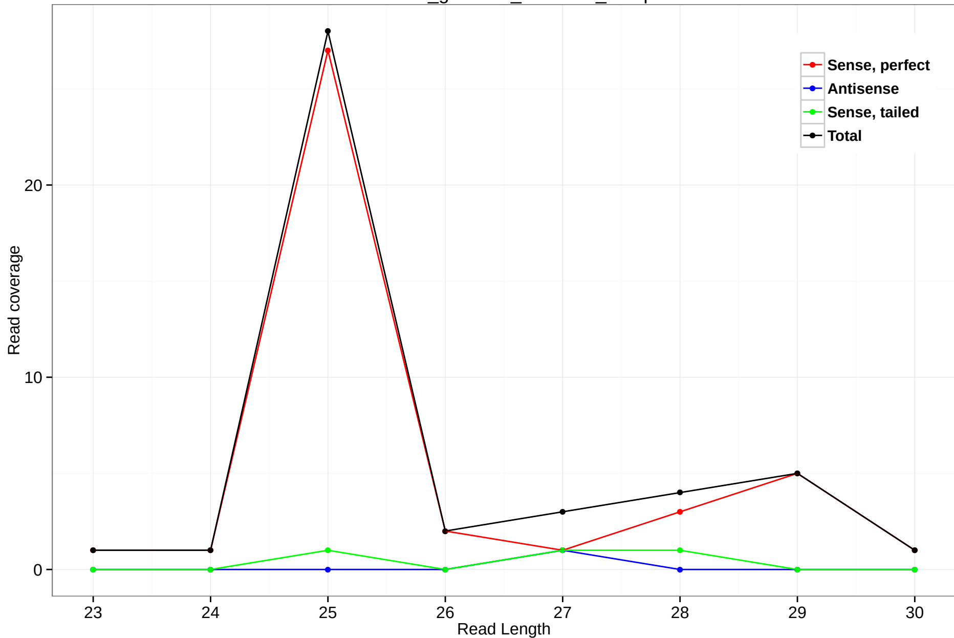
rheMac3_genscan_chr3.029_30.5p
