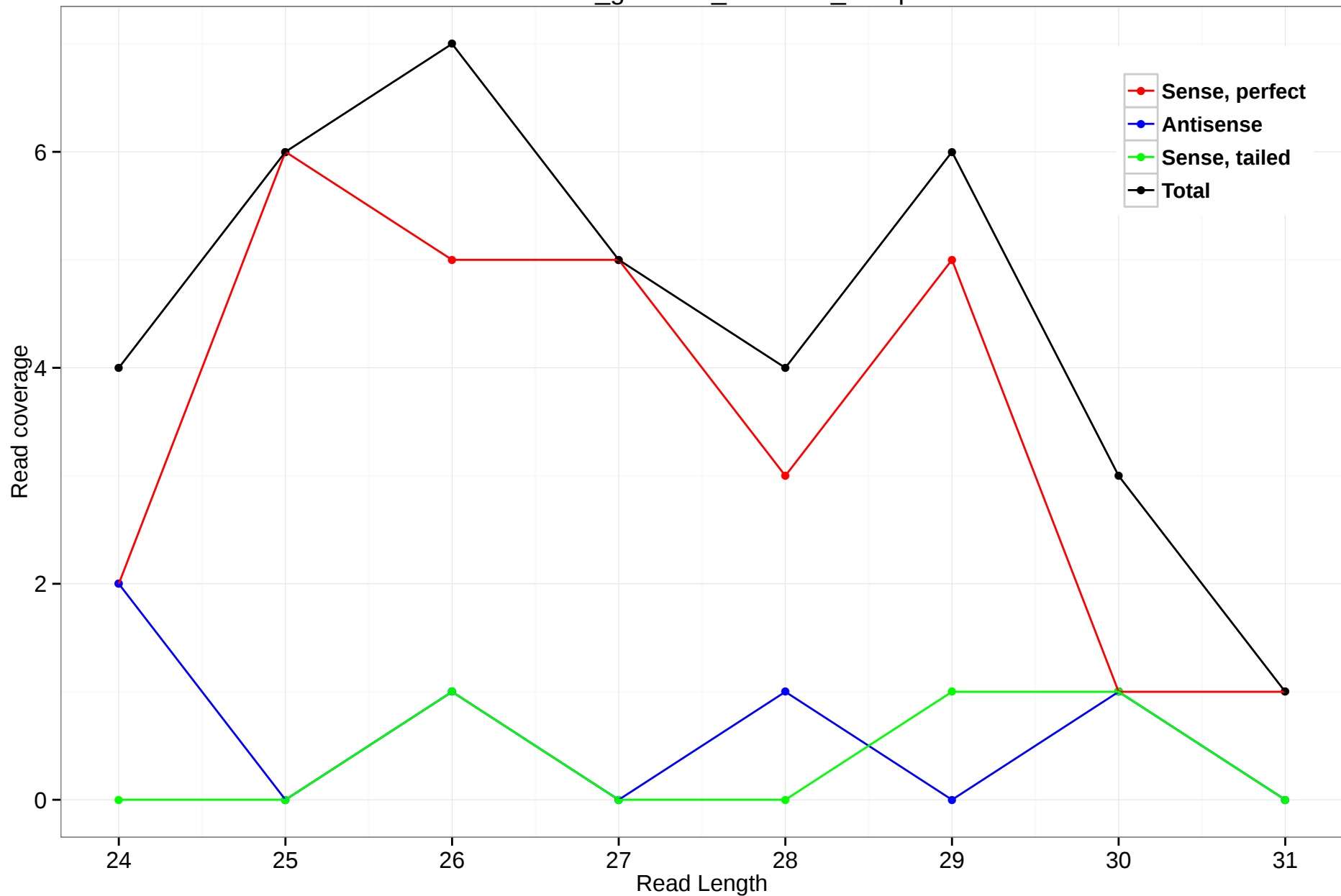
rheMac3_genscan_chr3.029_29.5p
