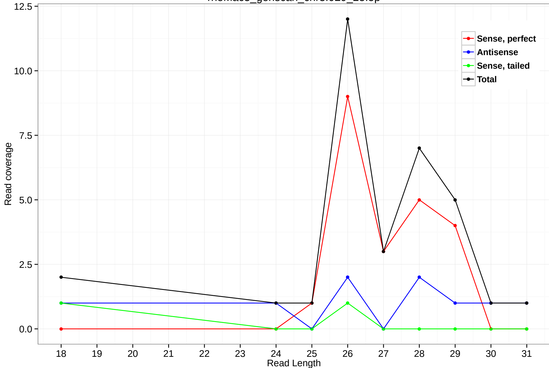
rheMac3_genscan_chr3.029_25.5p
