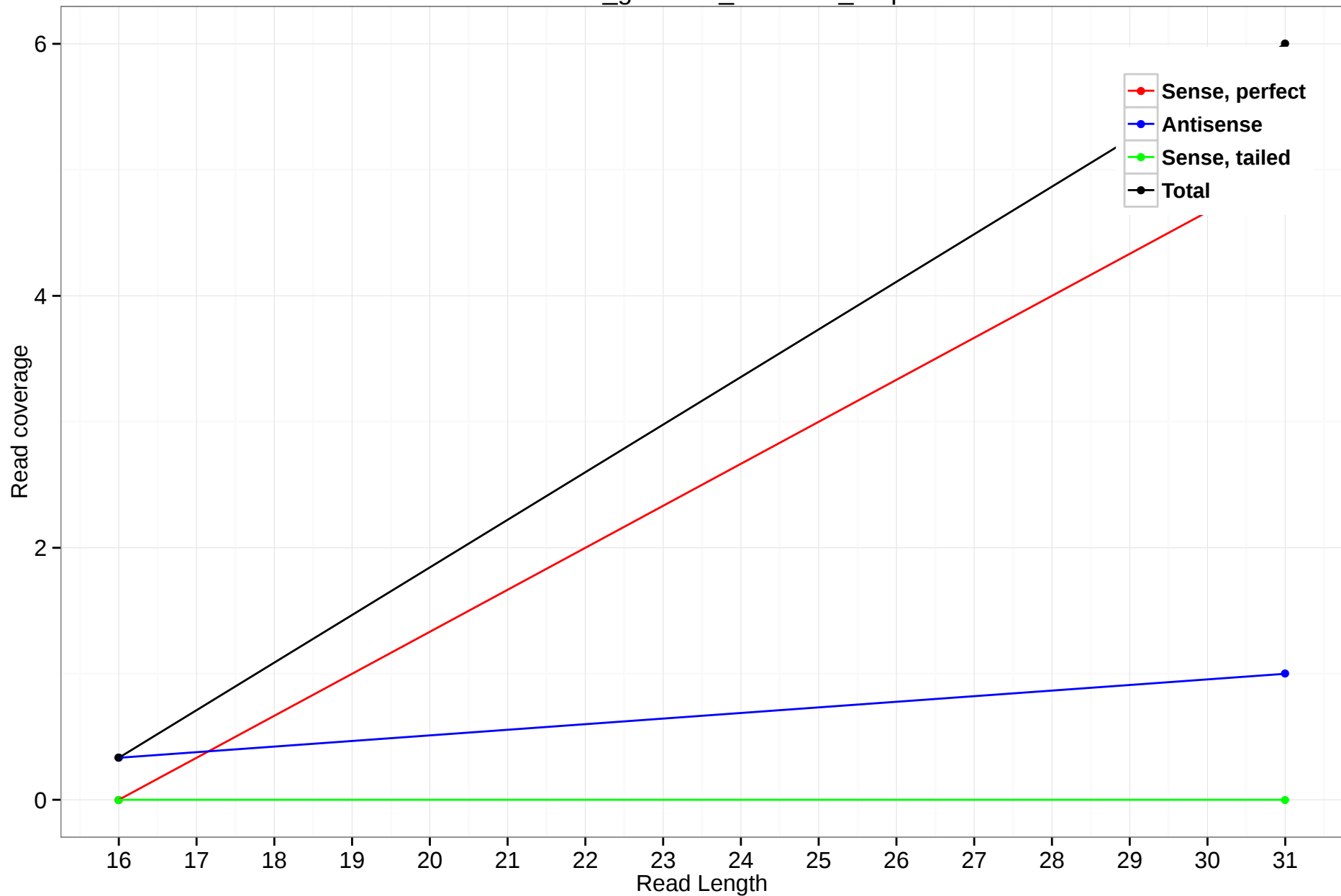
rheMac3_genscan_chr2.979_7.3p
