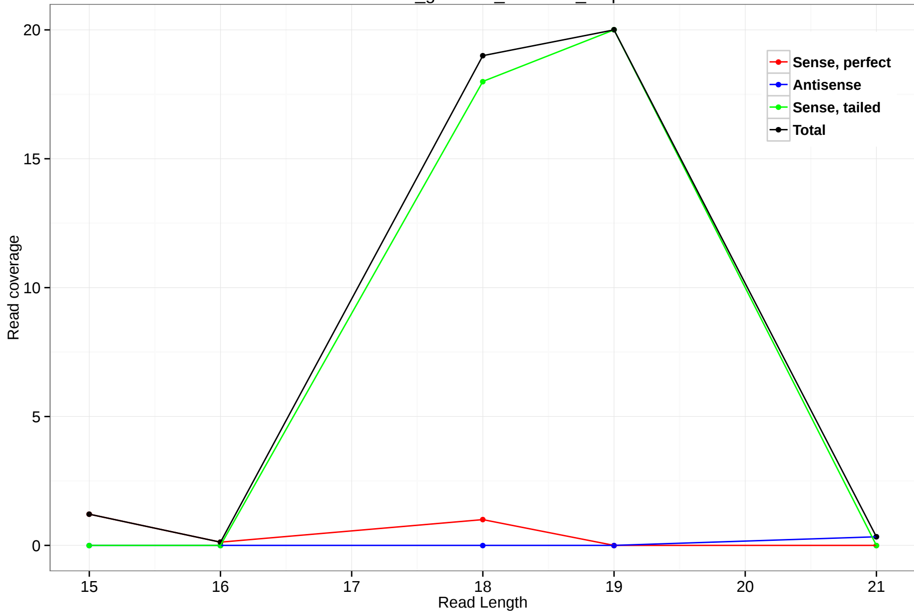
rheMac3_genscan_chr2.877_7.5p
