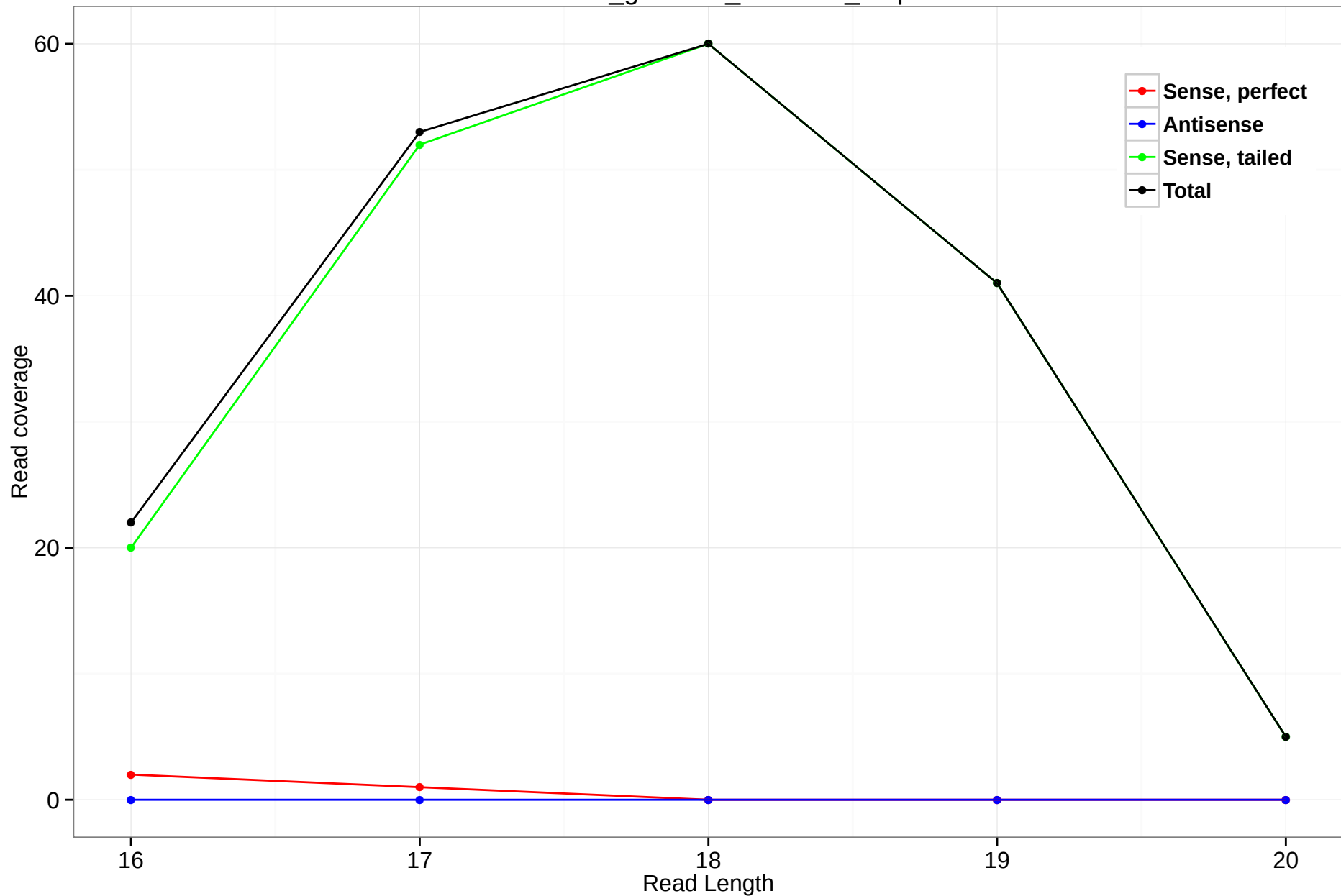
rheMac3_genscan_chr2.820_6.5p
