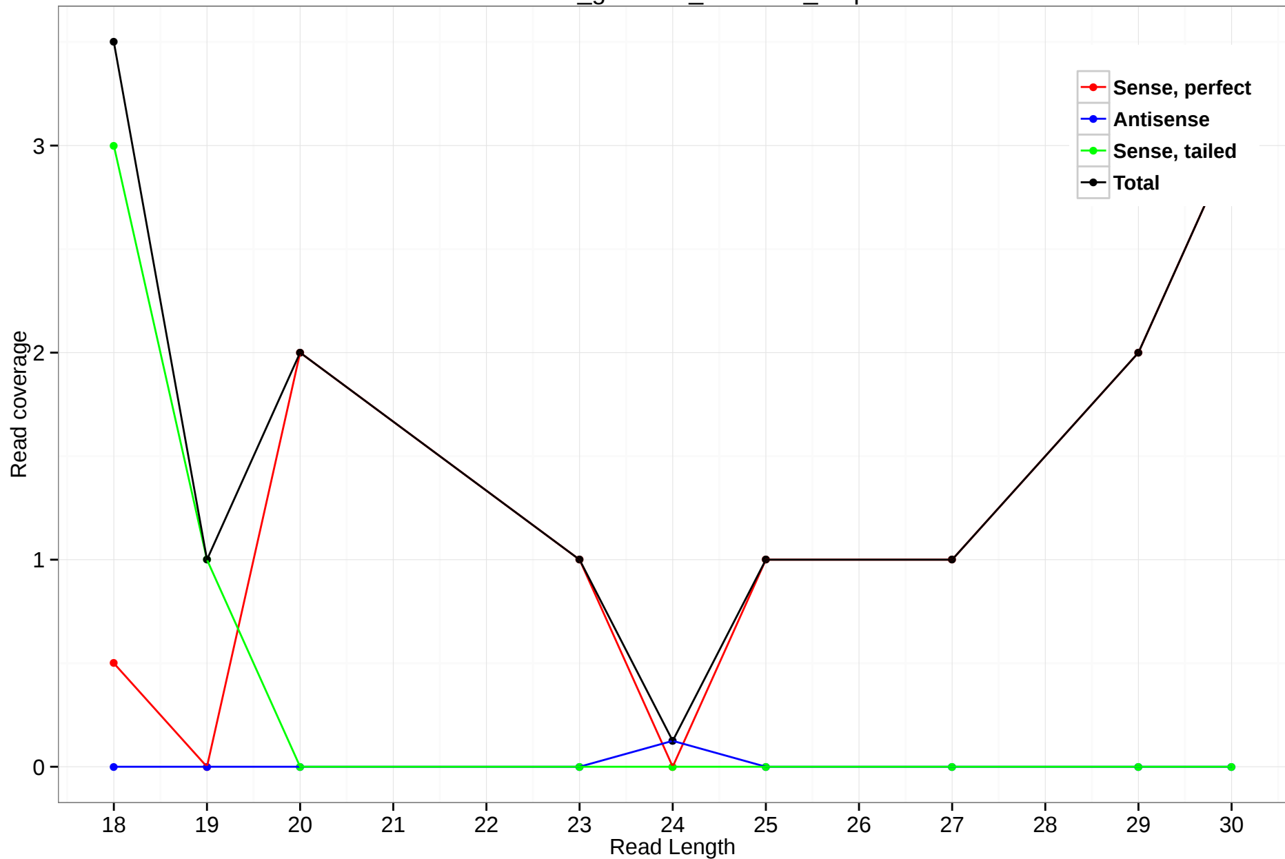
rheMac3_genscan_chr2.768_5.5p
