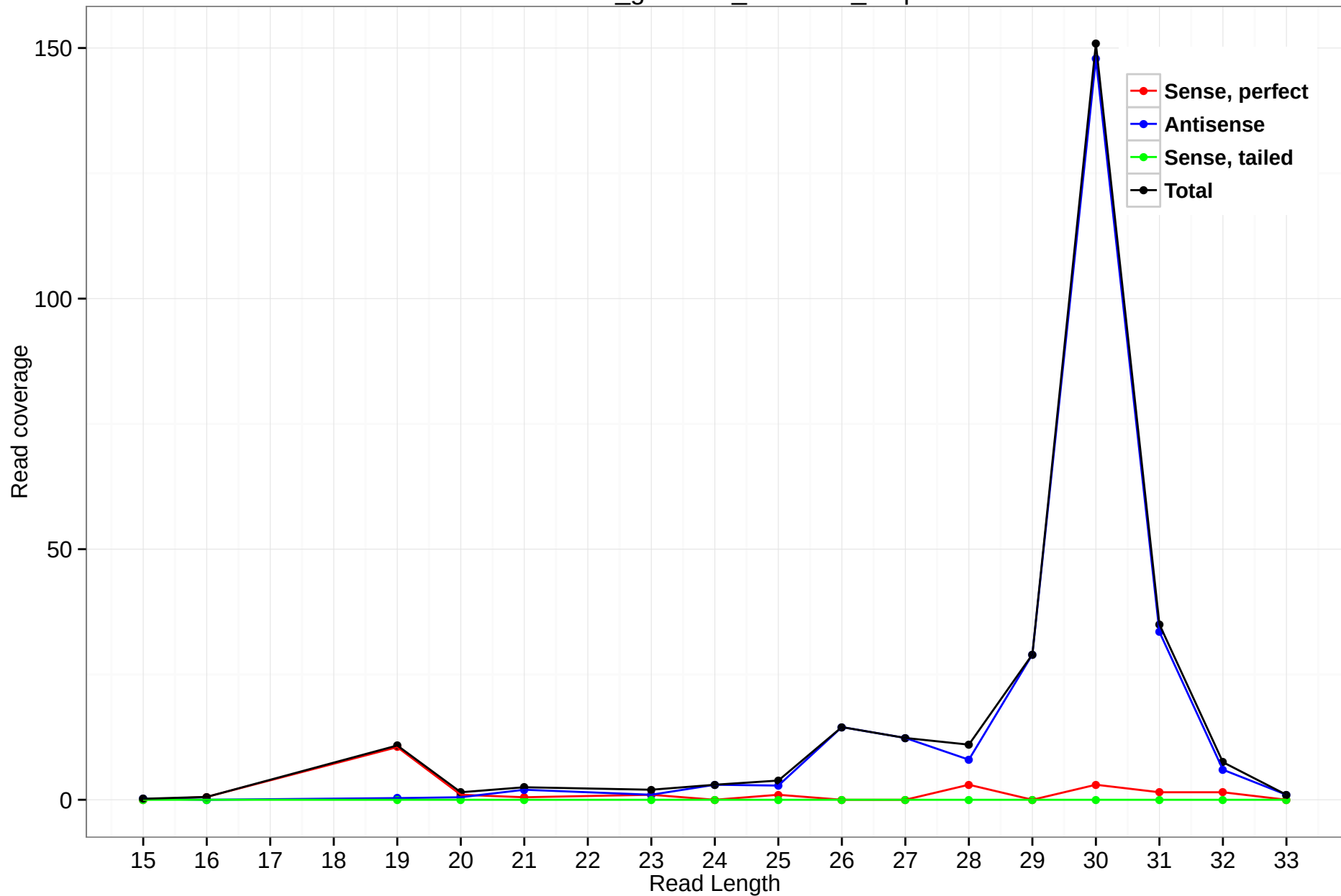
rheMac3_genscan_chr2.761_4.5p
