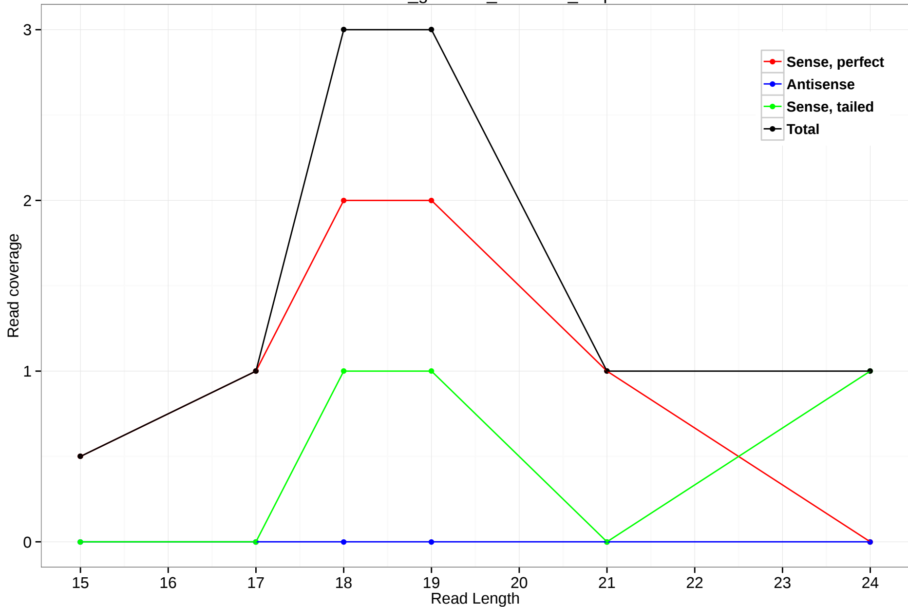
rheMac3_genscan_chr2.698_4.5p
