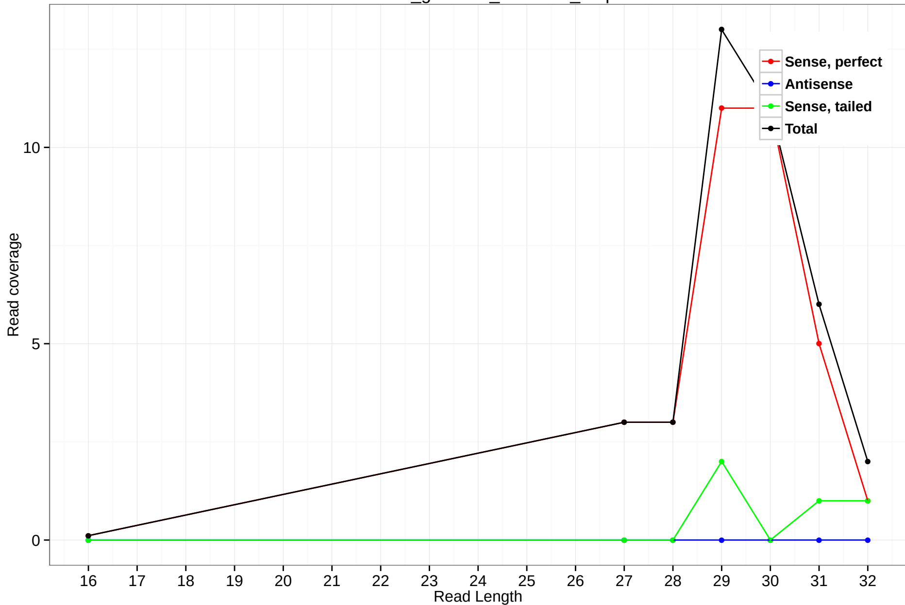
rheMac3_genscan_chr2.697_0.3p
