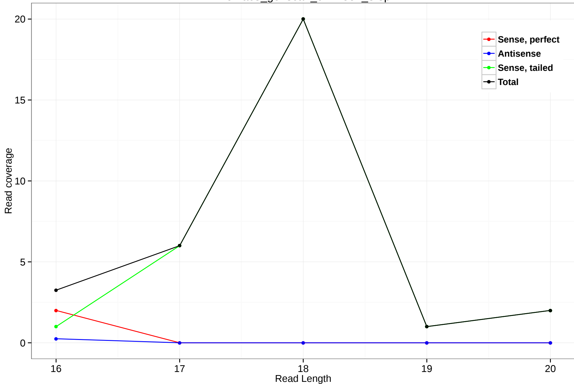
rheMac3_genscan_chr2.551_8.3p
