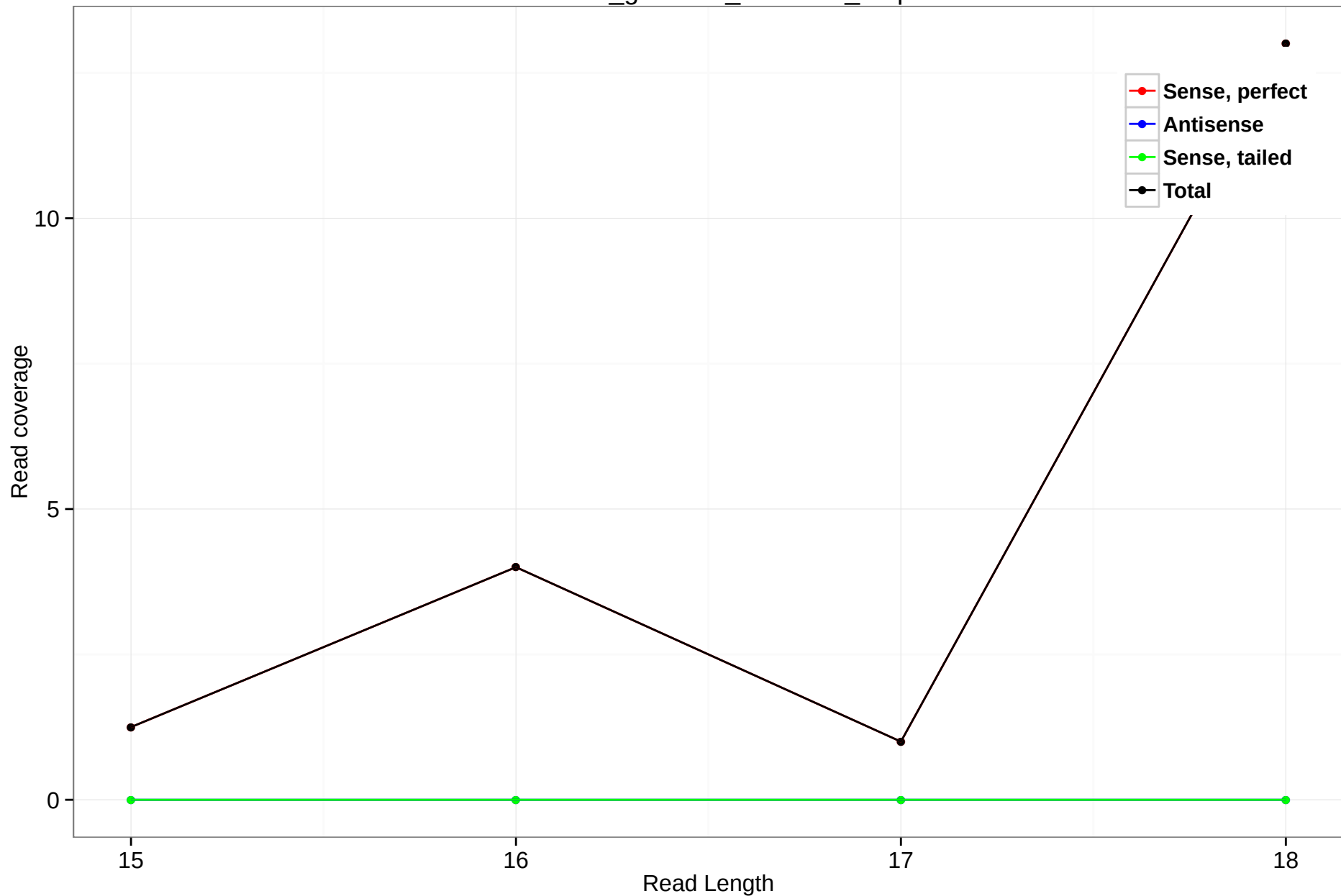
rheMac3_genscan_chr2.551_1.5p
