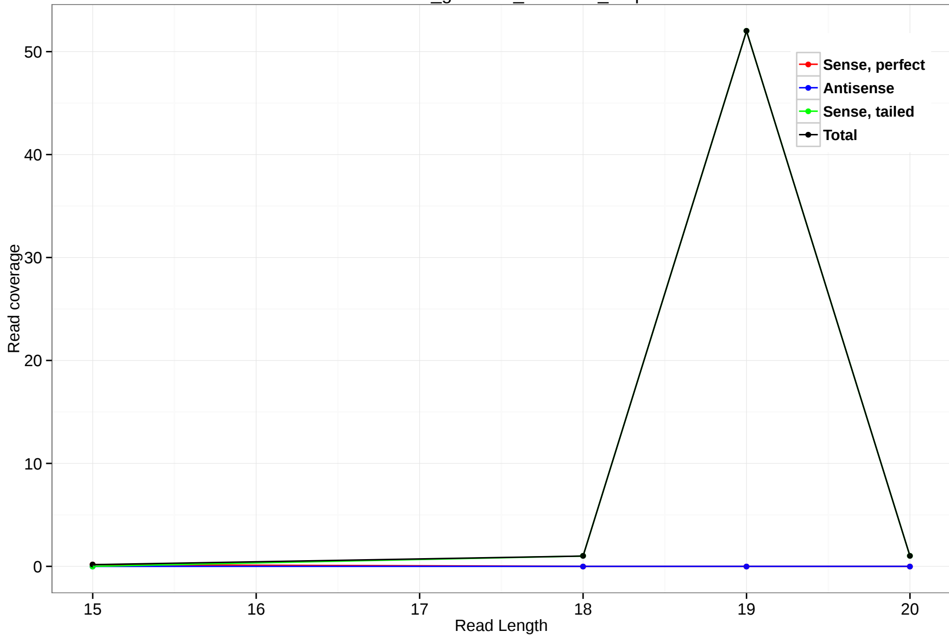
rheMac3_genscan_chr2.505_0.5p
