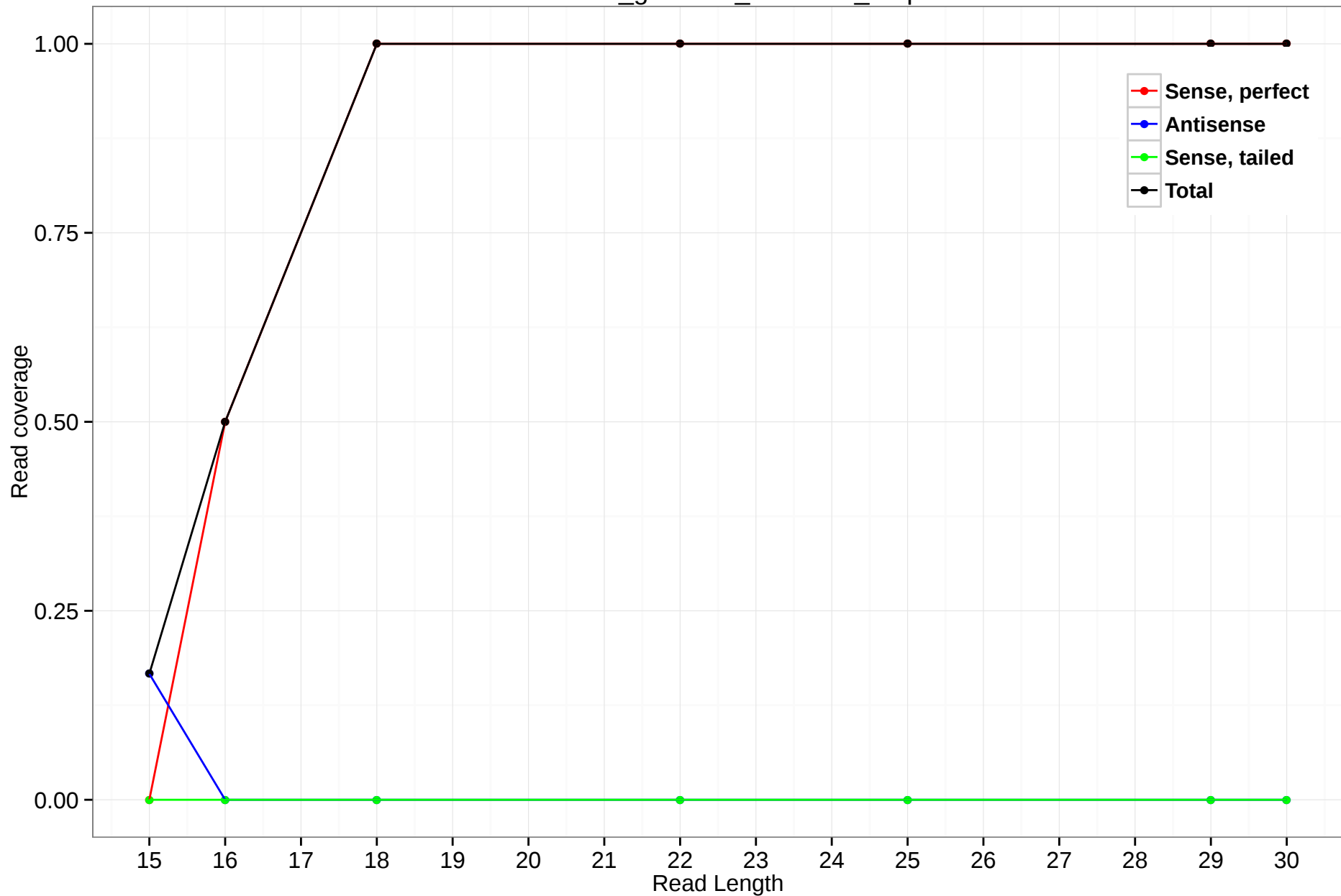
rheMac3_genscan_chr2.502_8.3p
