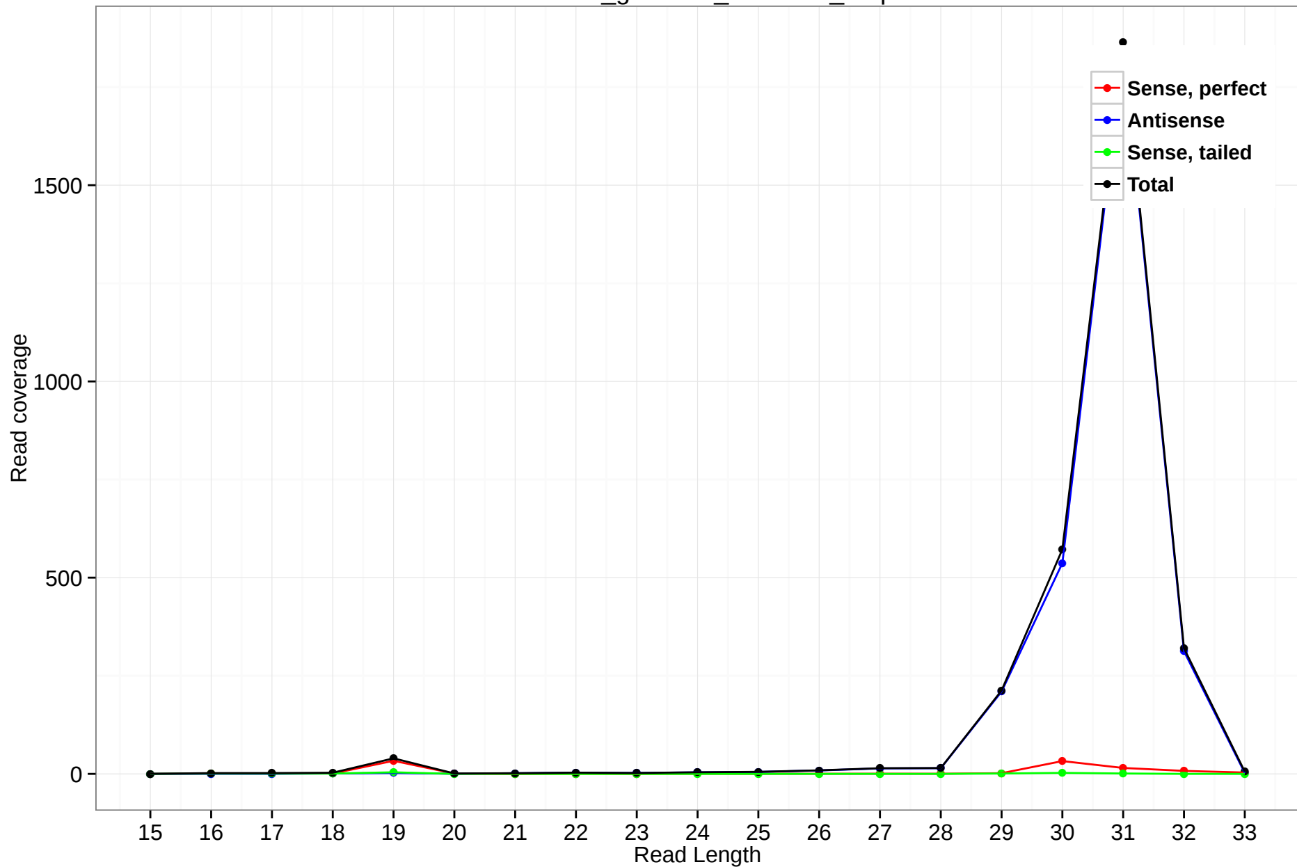
rheMac3_genscan_chr2.478_0.5p
