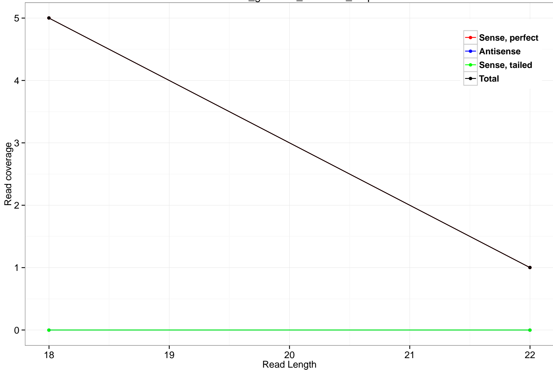
rheMac3_genscan_chr2.433_0.5p
