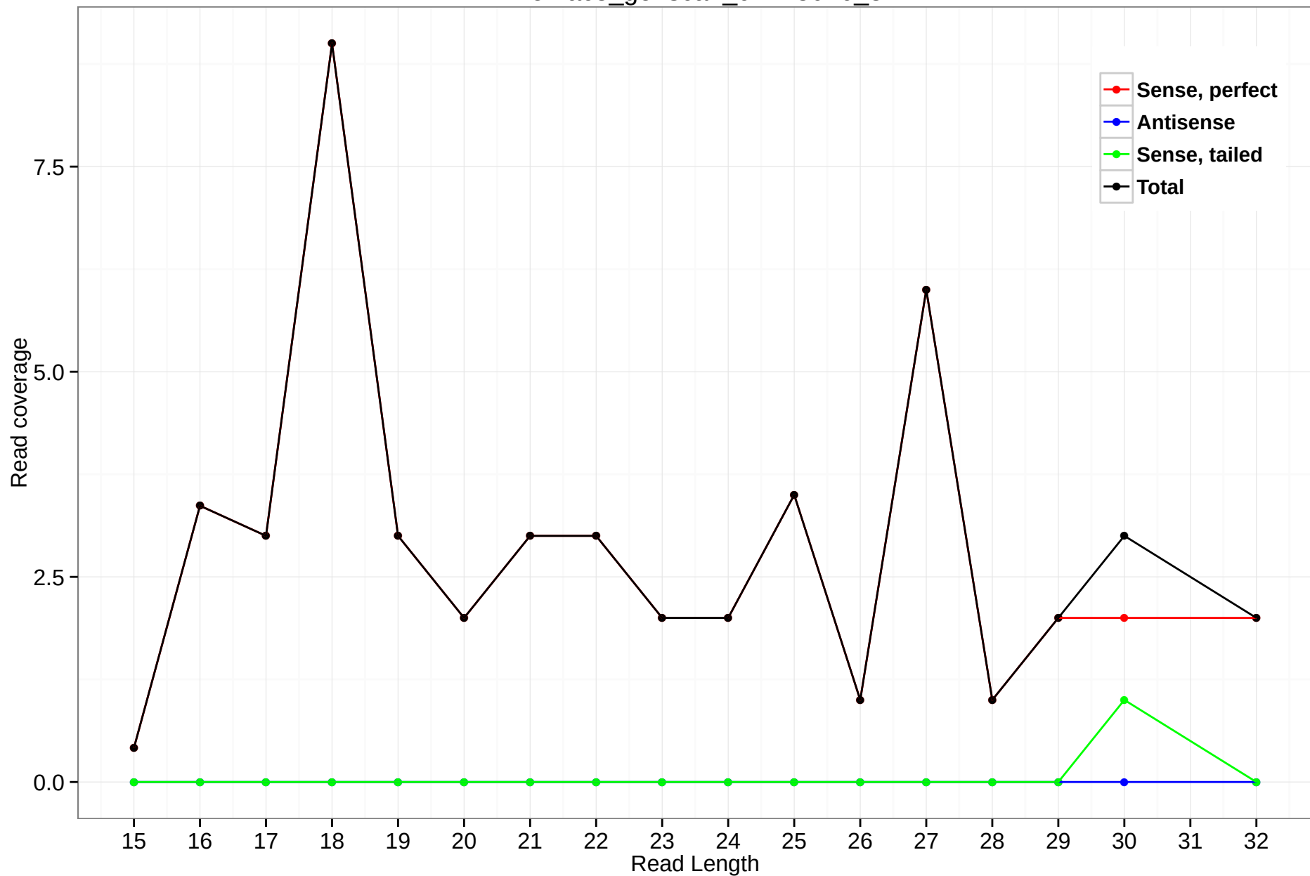
rheMac3_genscan_chr2.3076_8
