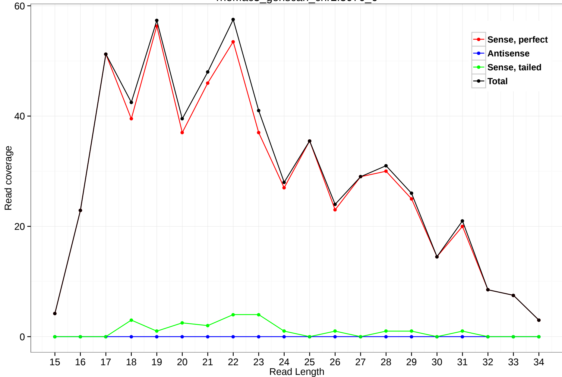
rheMac3_genscan_chr2.3076_6
