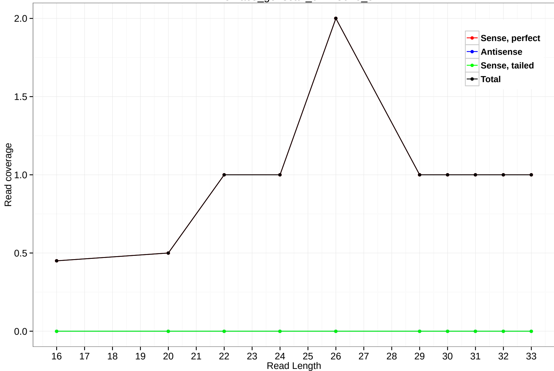
rheMac3_genscan_chr2.3076_5
