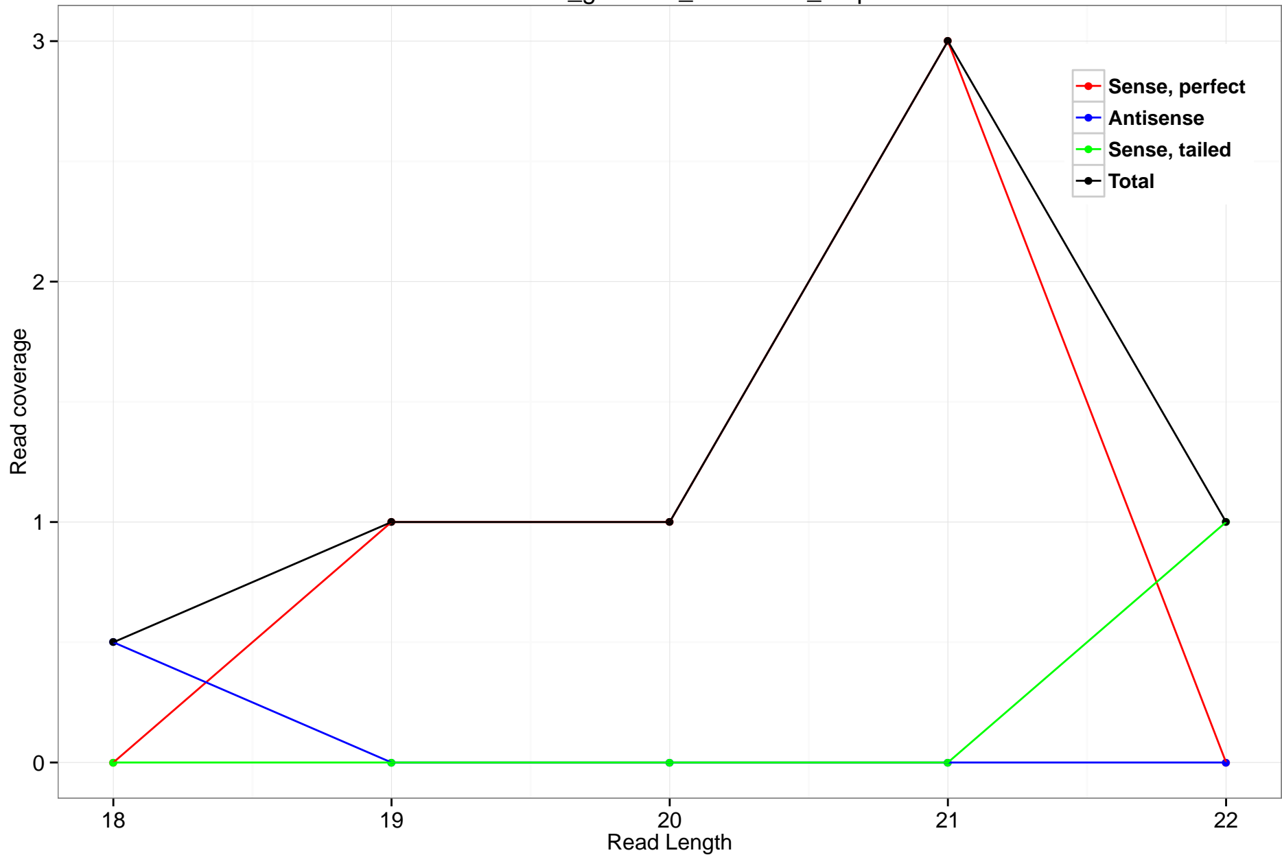
rheMac3_genscan_chr2.3041_2.5p
