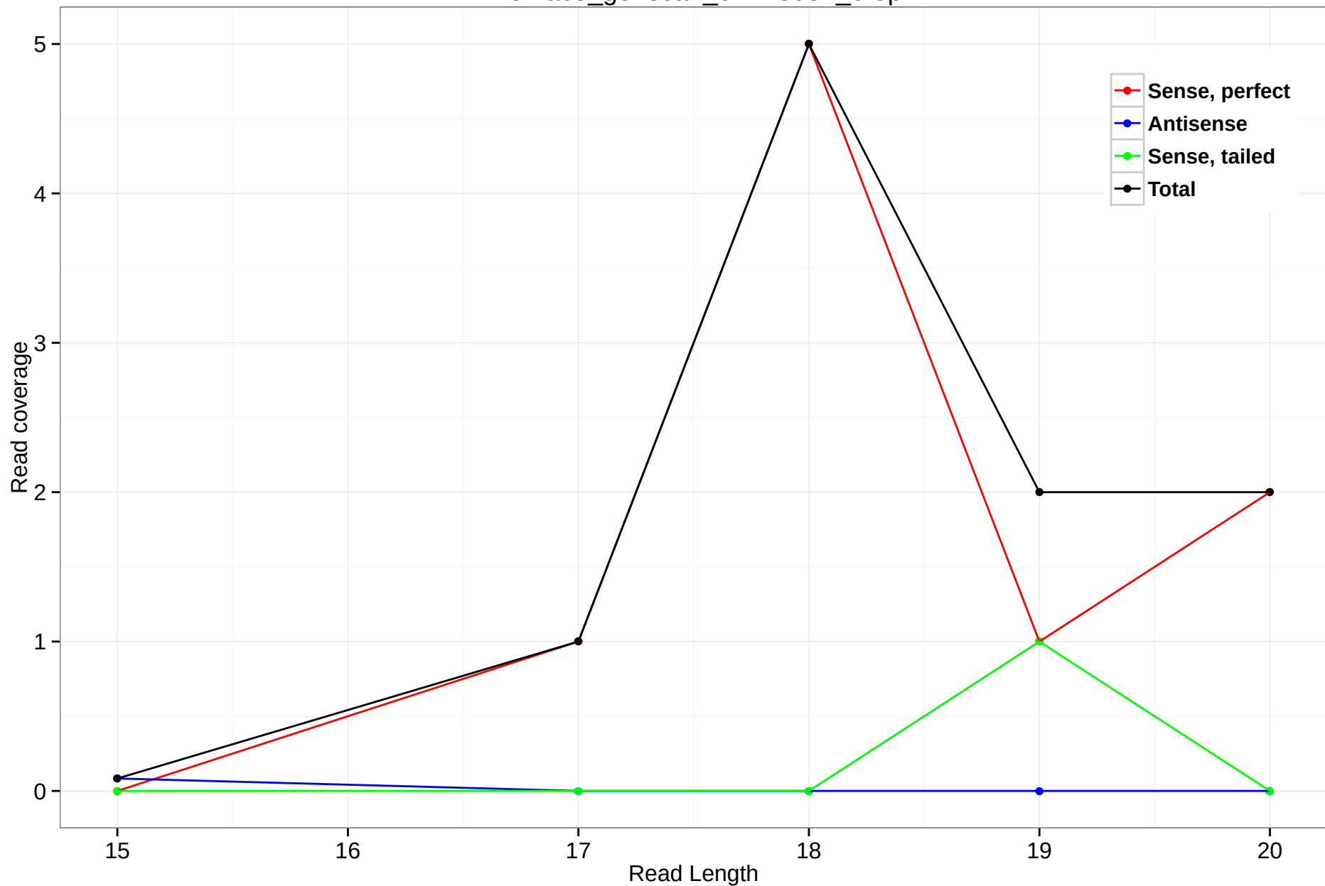
rheMac3_genscan_chr2.3032_0.3p
