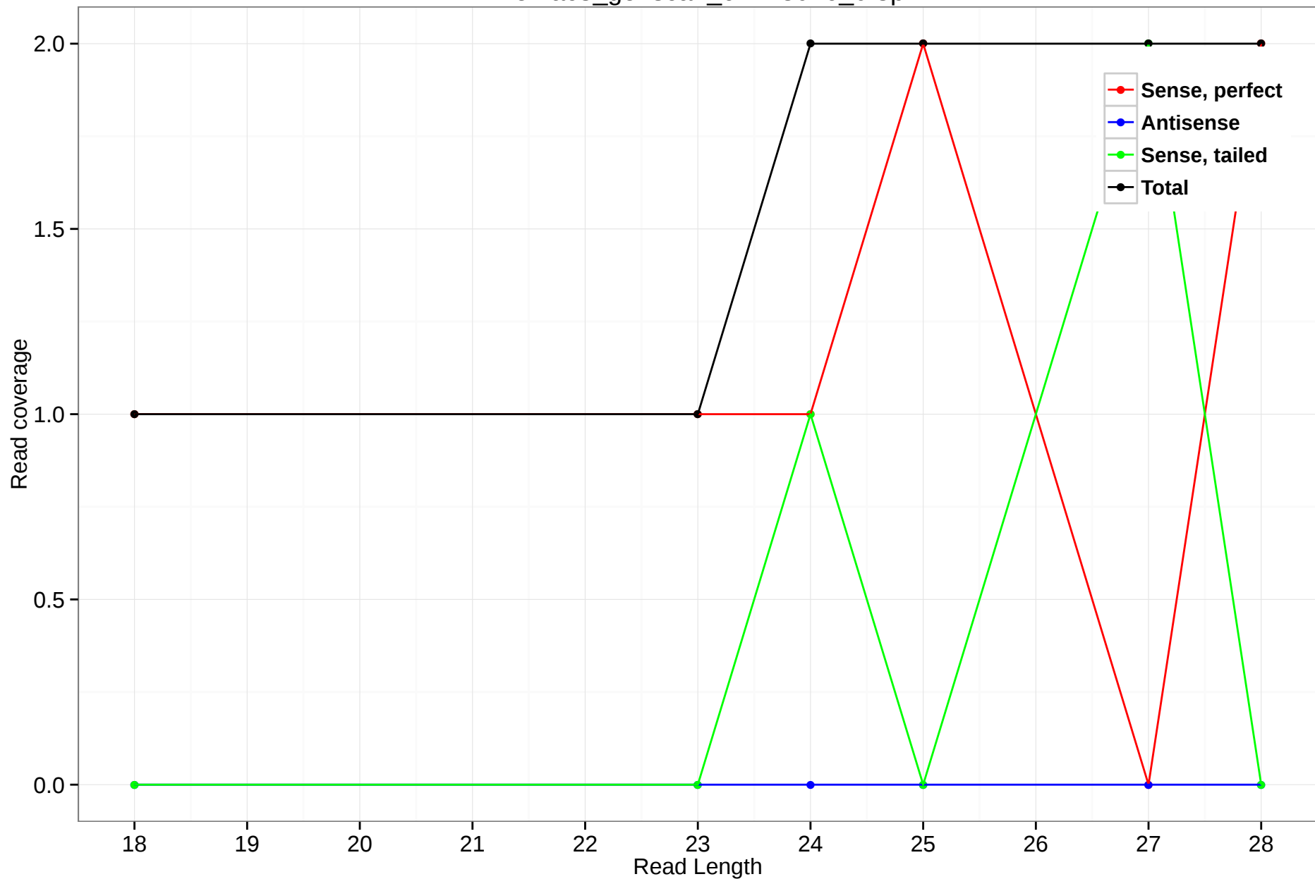
rheMac3_genscan_chr2.3016_0.3p
