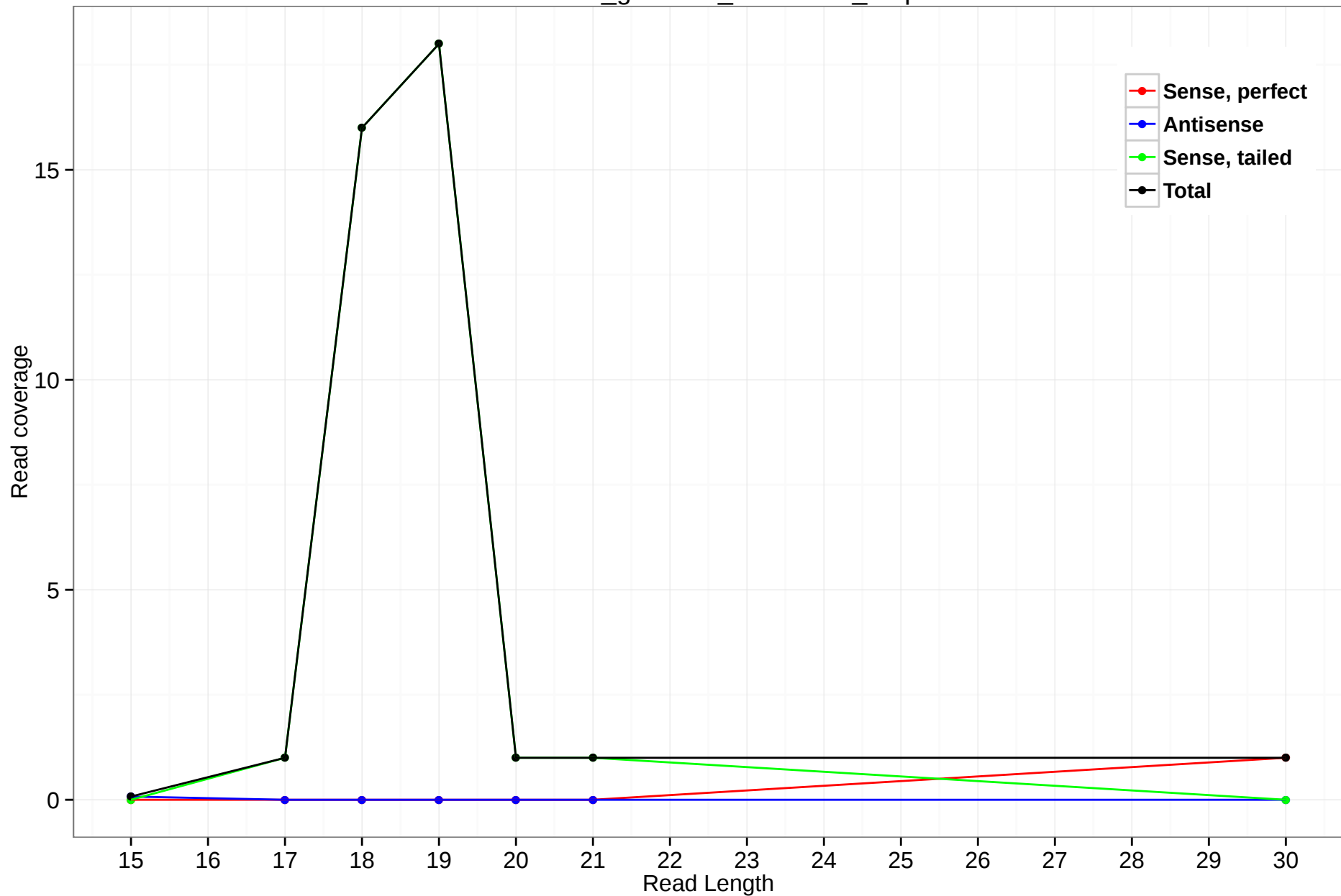
rheMac3_genscan_chr2.2914_3.3p
