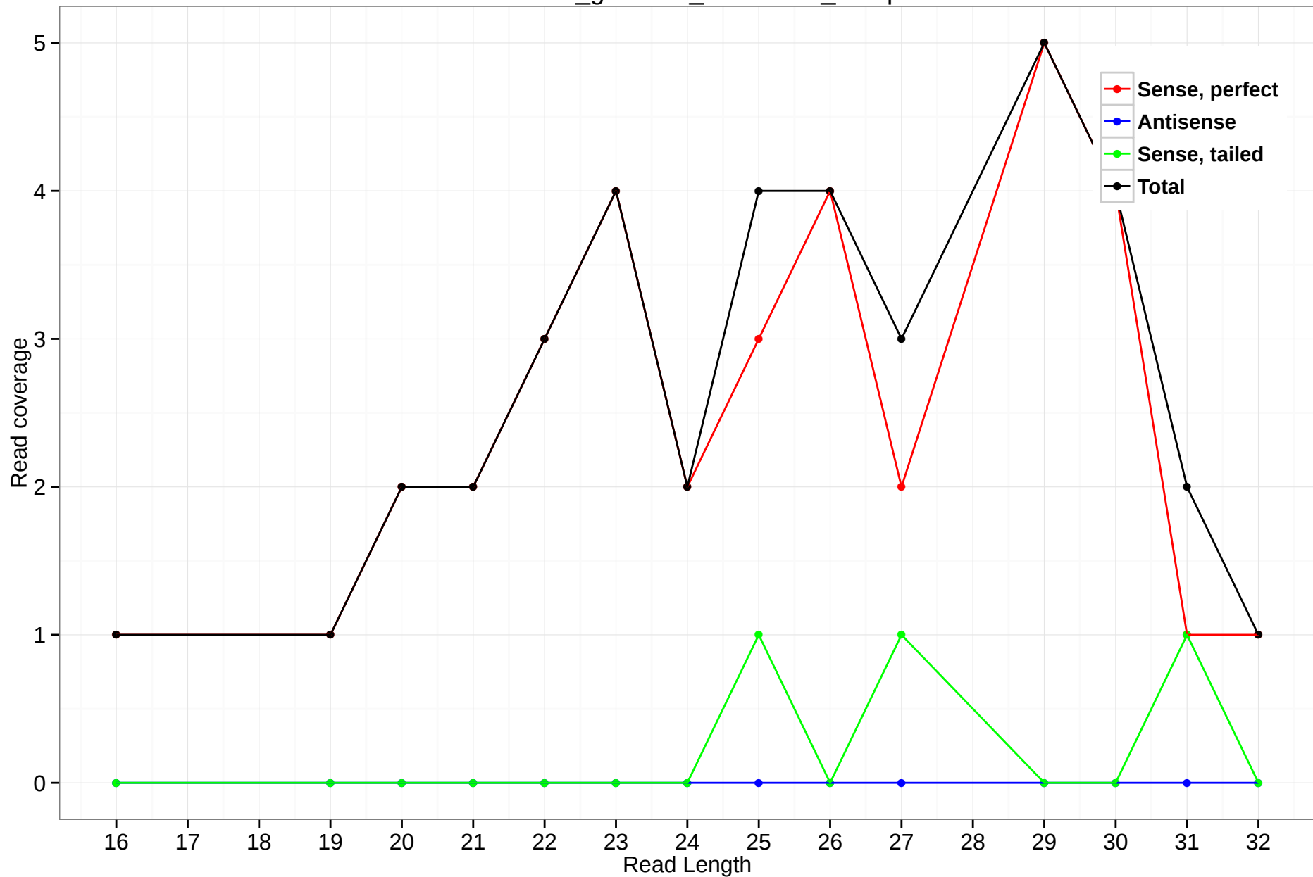
rheMac3_genscan_chr2.2757_17.3p
