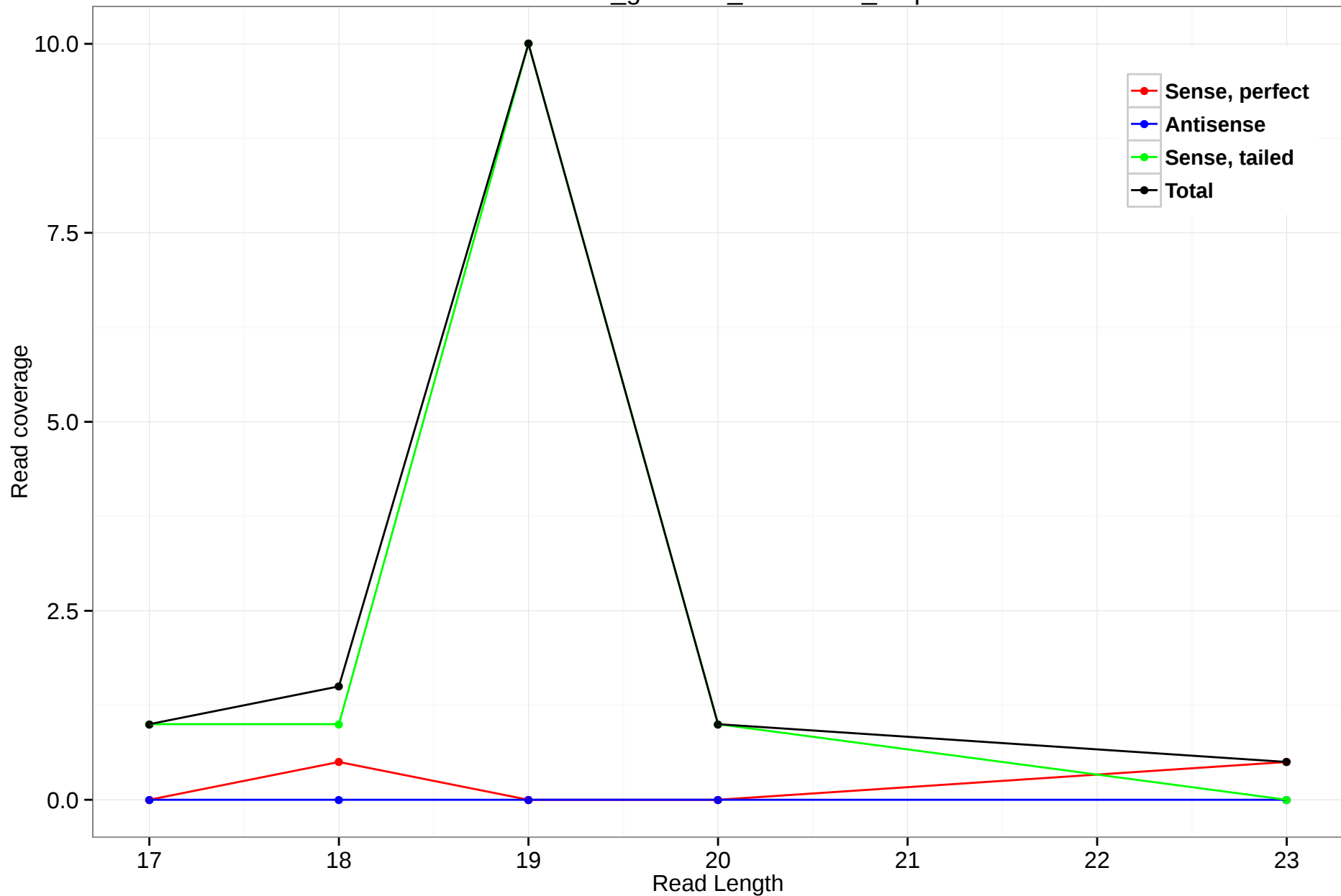
rheMac3_genscan_chr2.2689_3.5p
