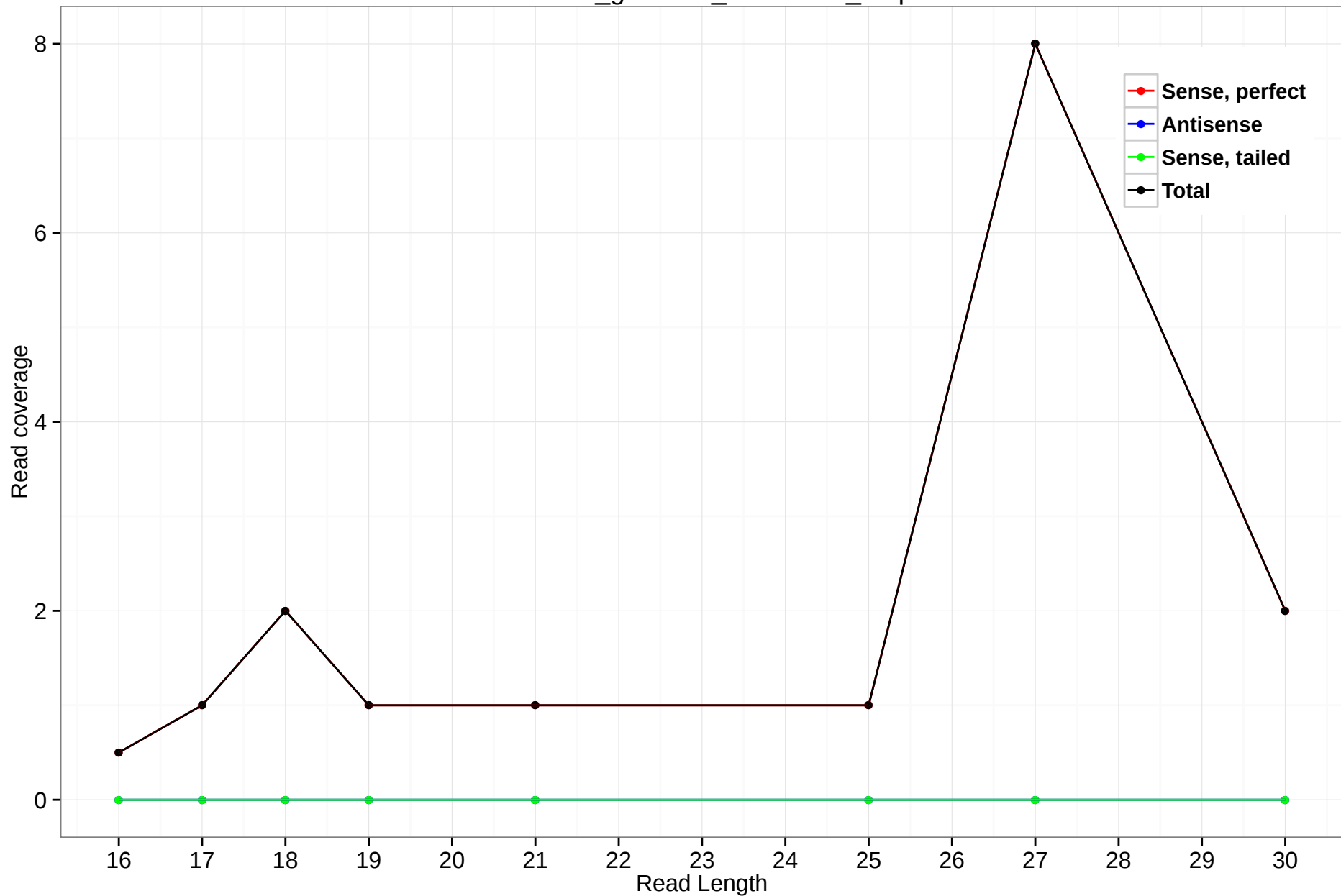
rheMac3_genscan_chr2.2673_1.5p
