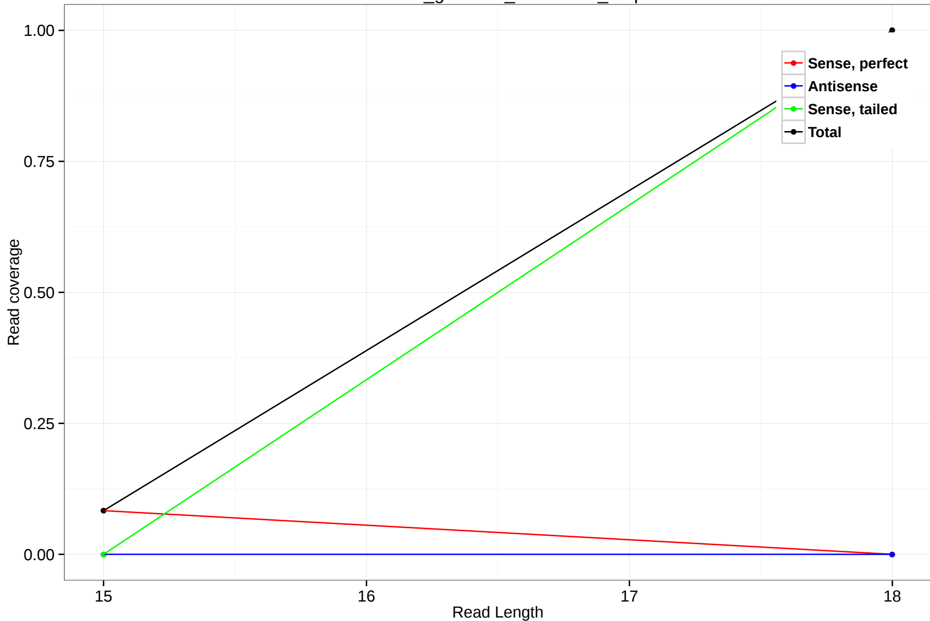
rheMac3_genscan_chr2.2629_8.3p
