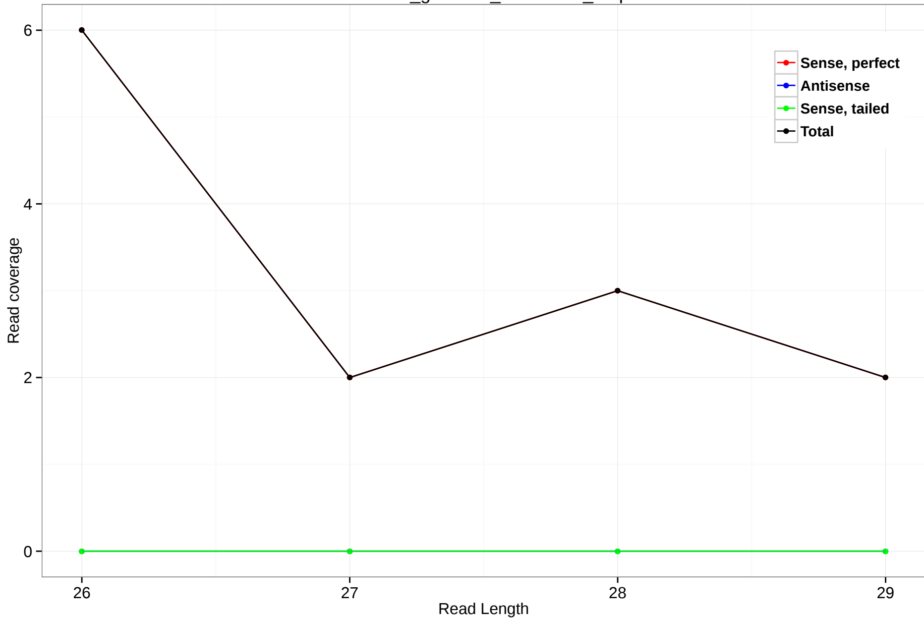
rheMac3_genscan_chr2.2628_6.5p
