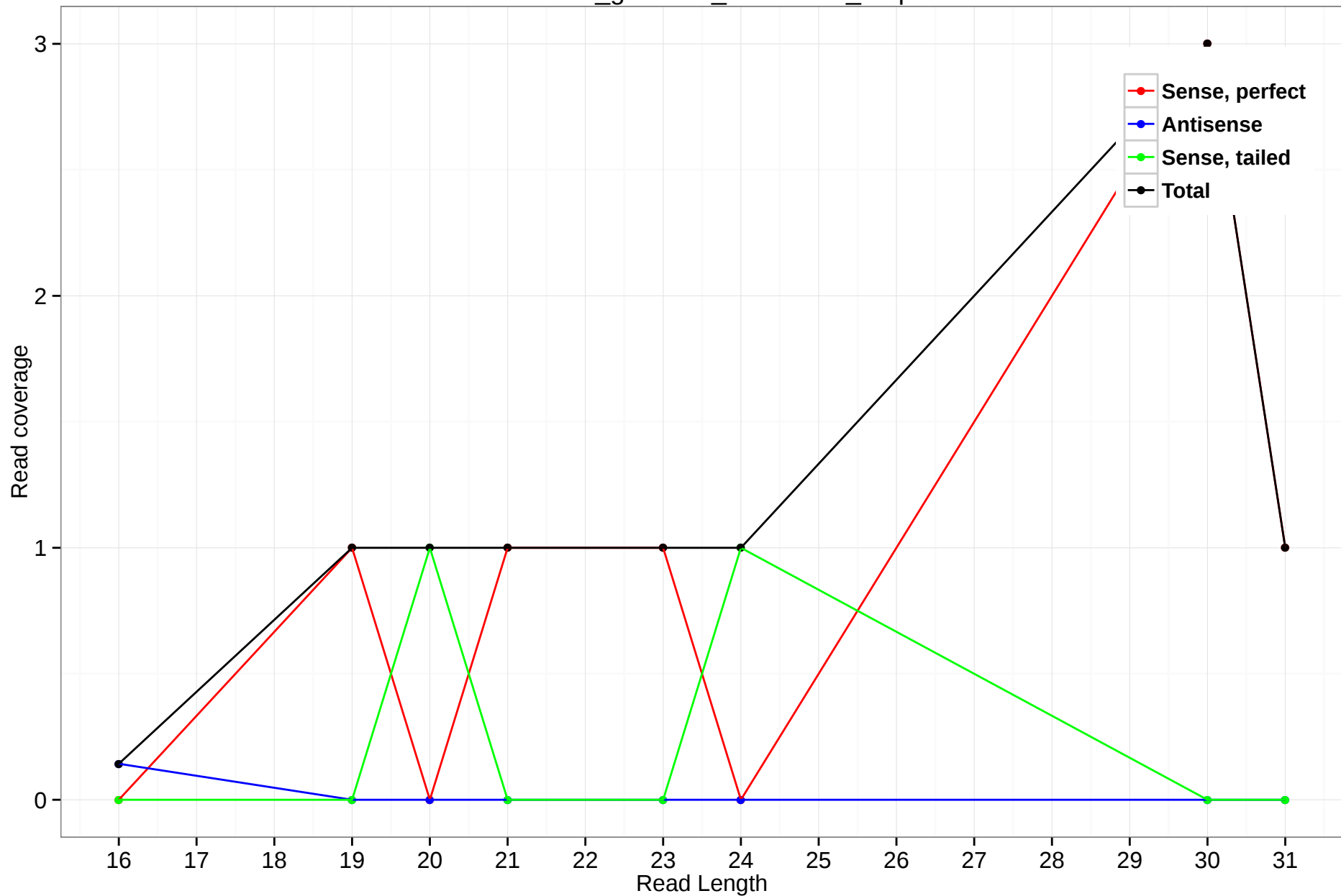
rheMac3_genscan_chr2.2584_0.3p
