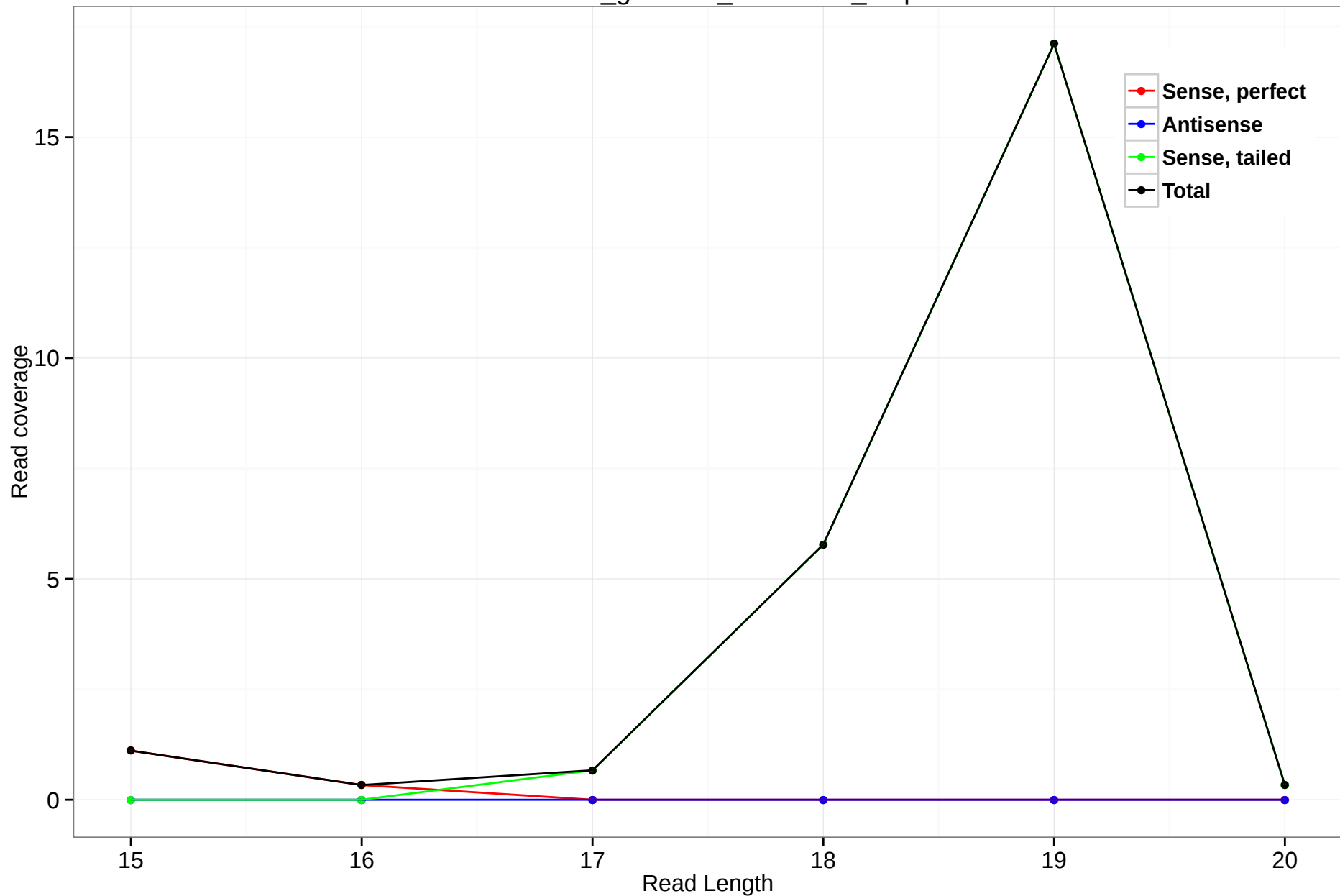
rheMac3_genscan_chr2.2563_3.3p
