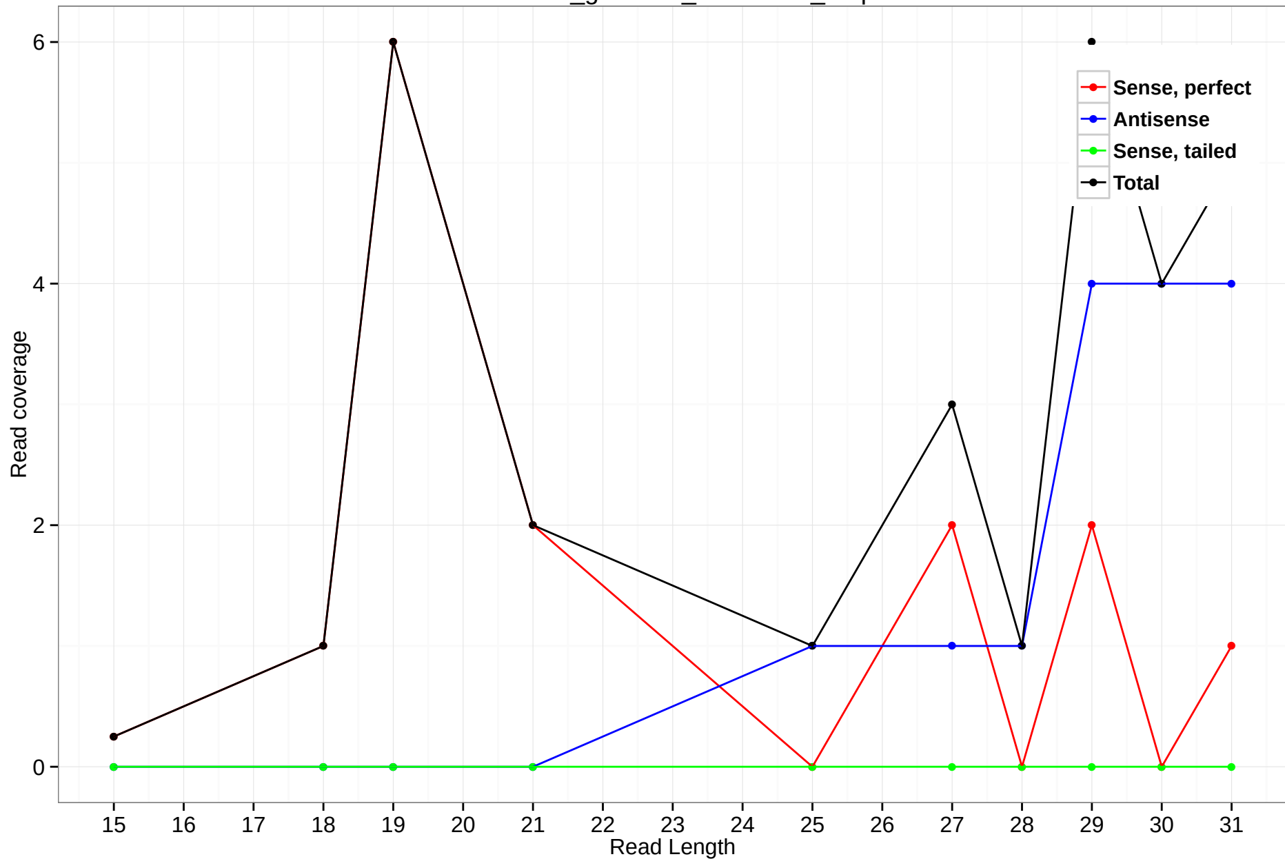
rheMac3_genscan_chr2.2537_7.5p
