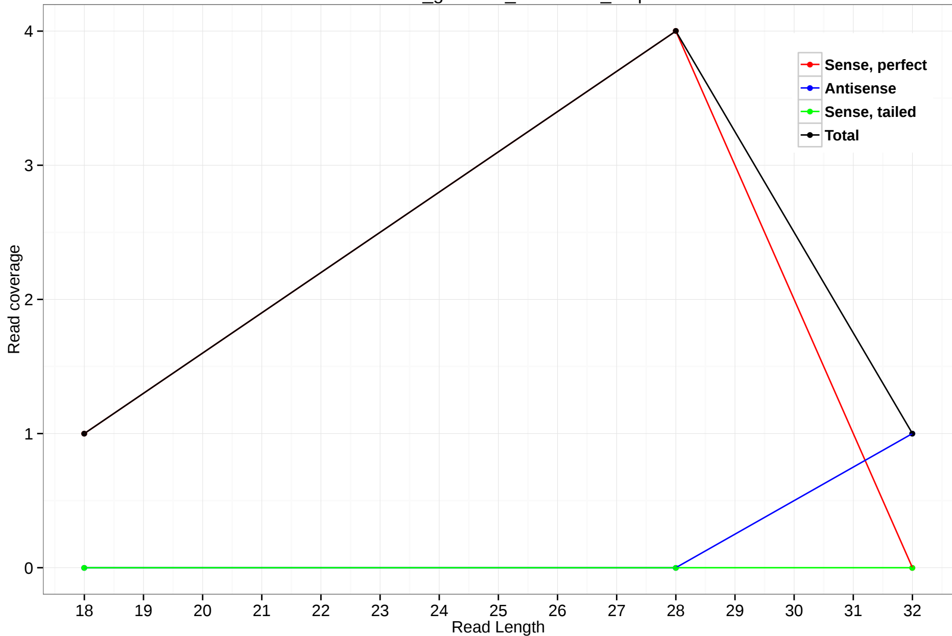
rheMac3_genscan_chr2.2537_7.3p
