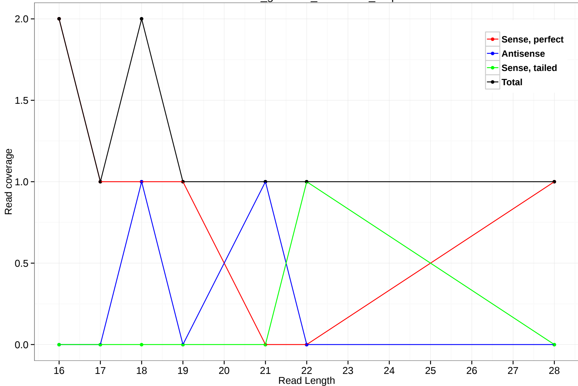
rheMac3_genscan_chr2.2488_3.5p
