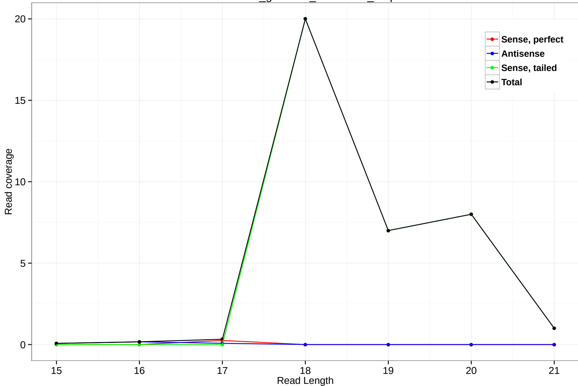
rheMac3_genscan_chr2.2404_7.5p
