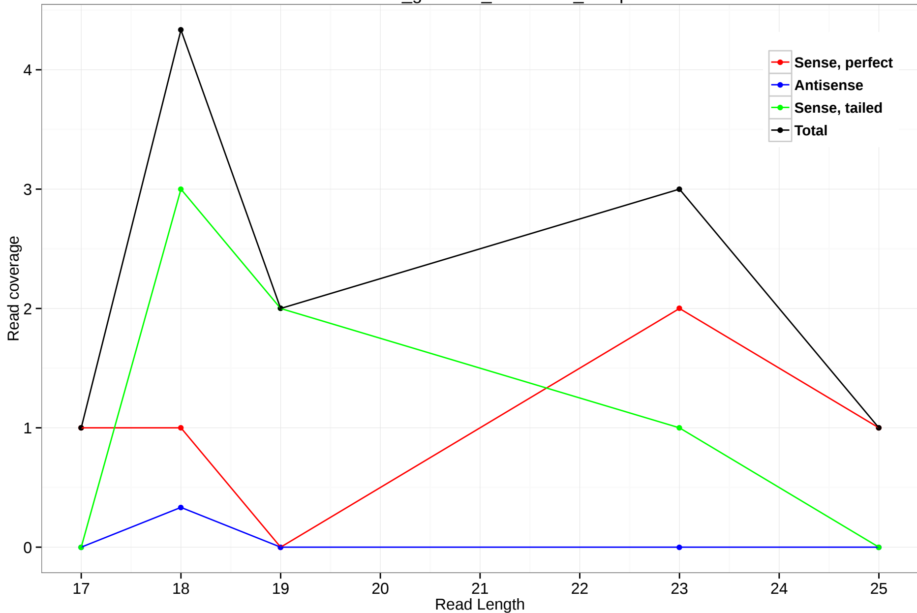
rheMac3_genscan_chr2.2381_10.5p
