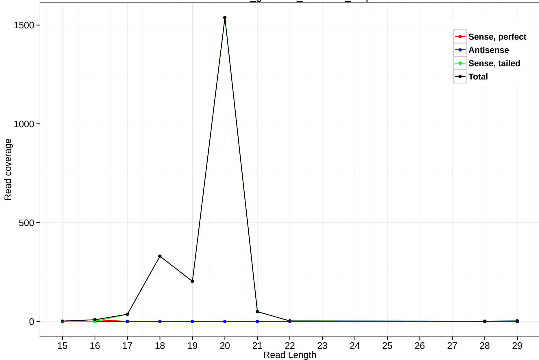
rheMac3_genscan_chr2.227_1.5p
