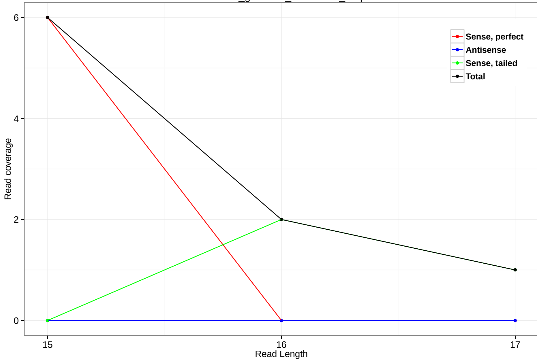
rheMac3_genscan_chr2.2248_0.5p
