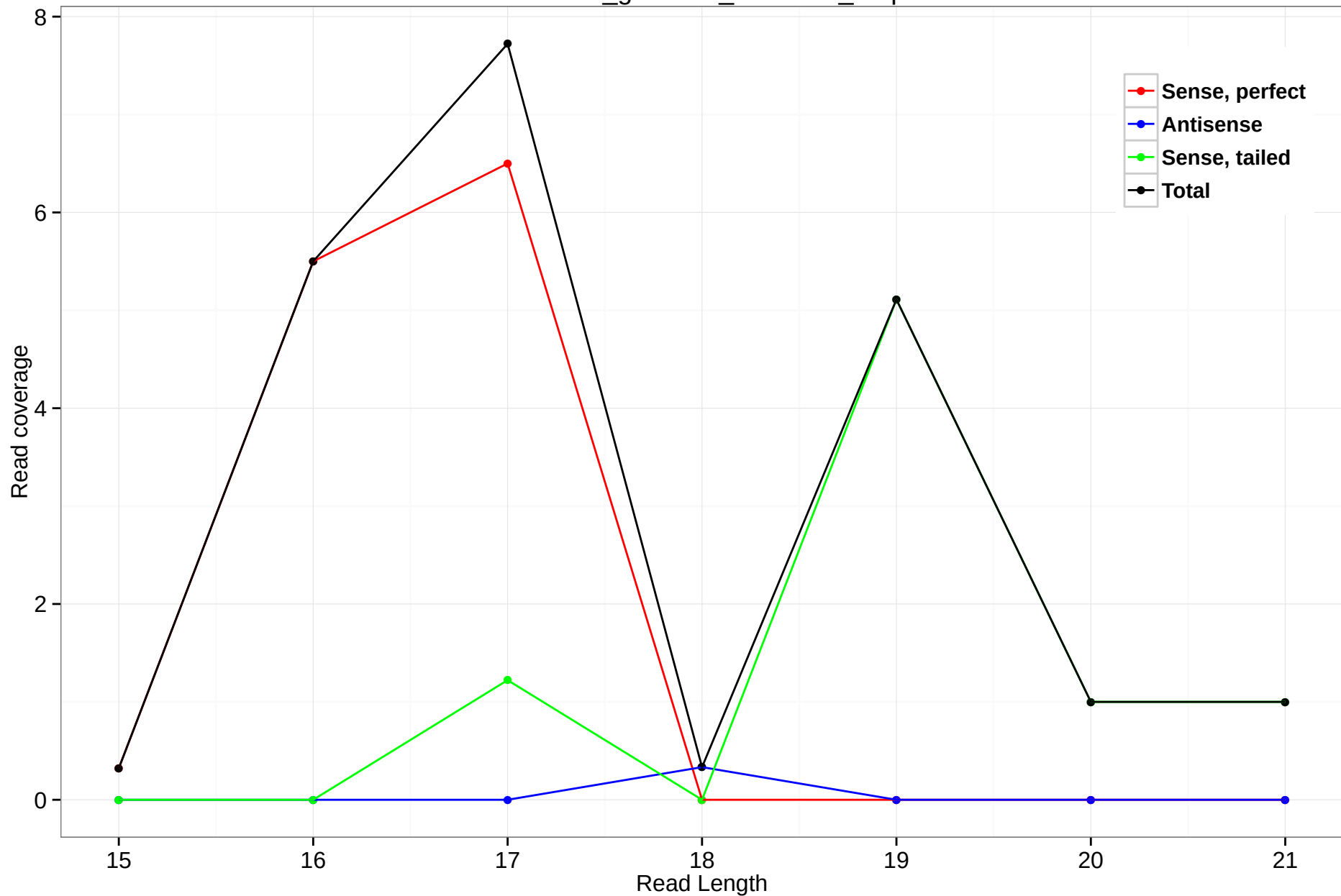
rheMac3_genscan_chr2.214_6.5p
