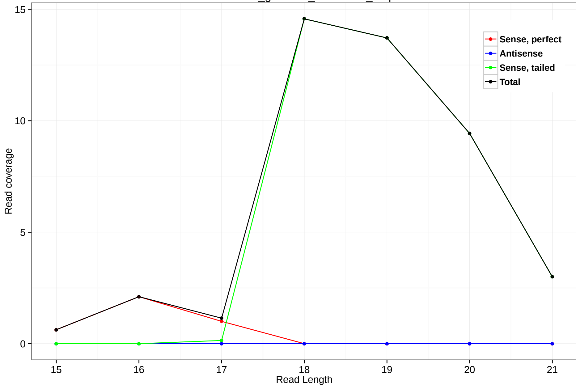
rheMac3_genscan_chr2.2057_1.5p
