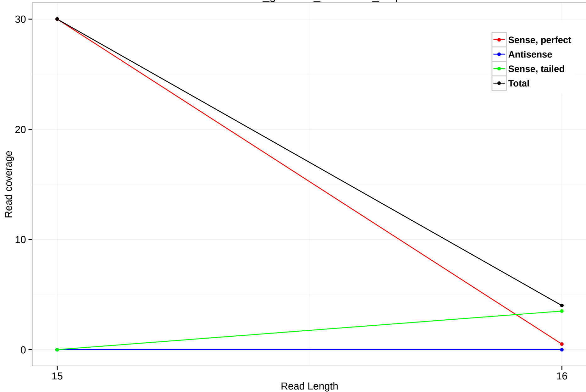
rheMac3_genscan_chr2.2015_2.5p
