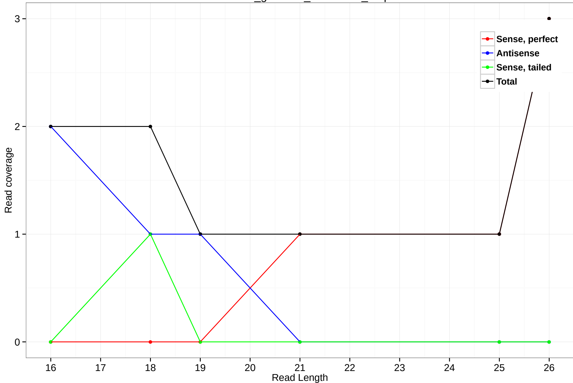
rheMac3_genscan_chr2.1967_1.3p
