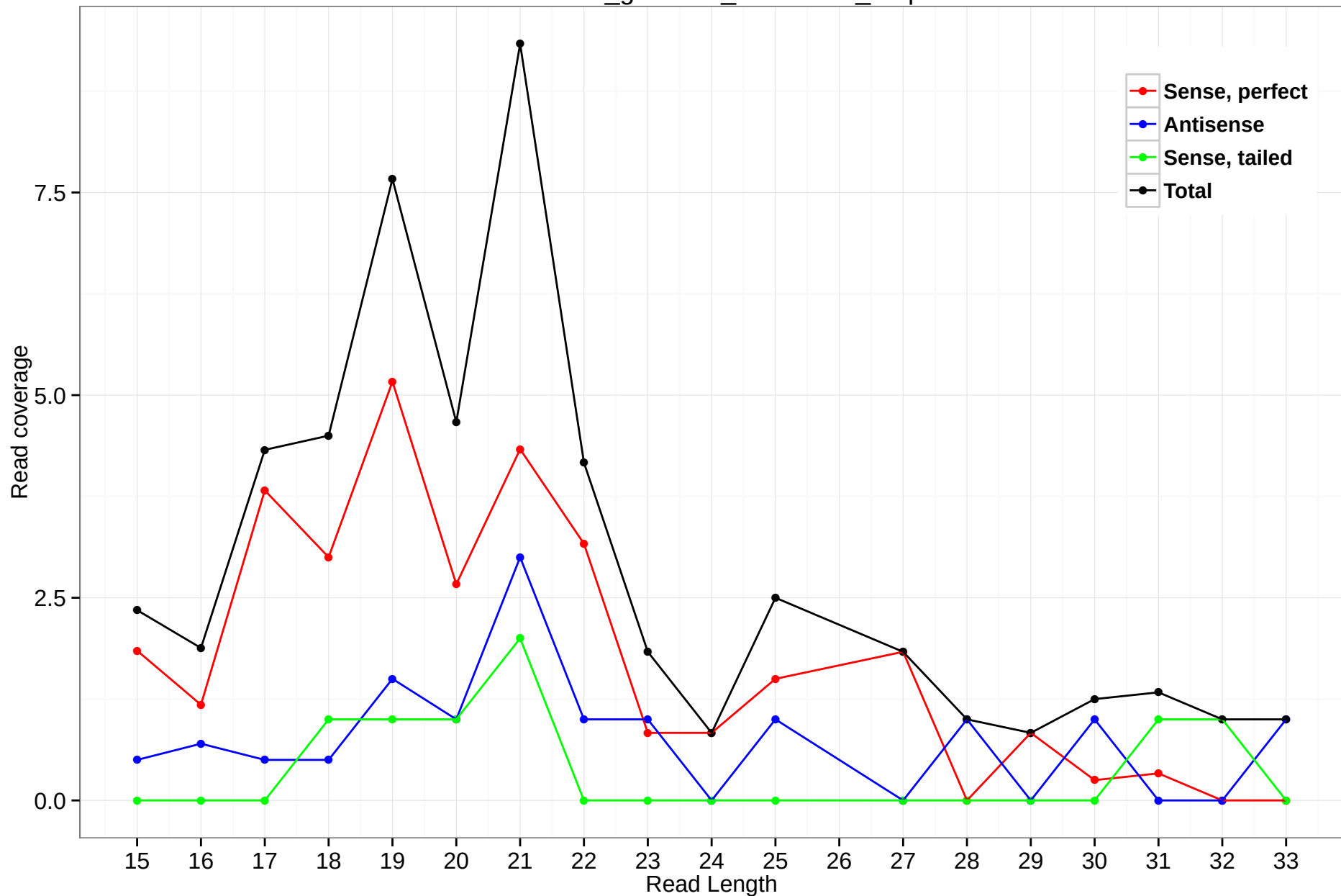
rheMac3_genscan_chr2.1947_0.5p
