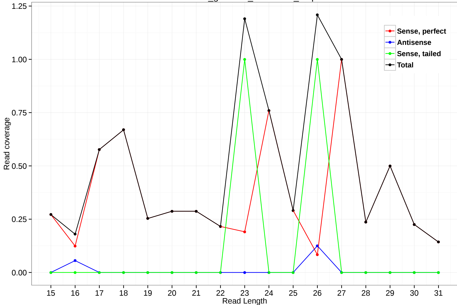
rheMac3_genscan_chr2.1794_0.5p
