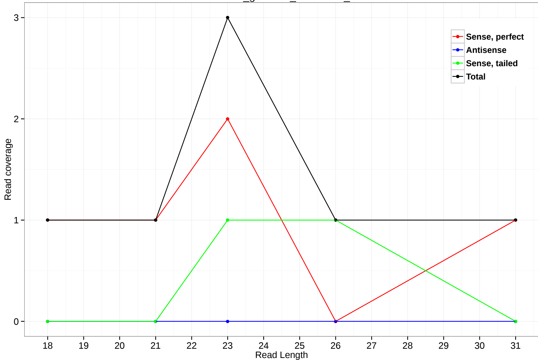
rheMac3_genscan_chr2.1792_27
