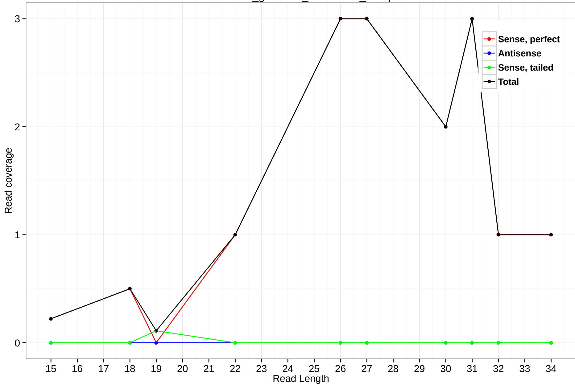
rheMac3_genscan_chr2.1758_13.5p
