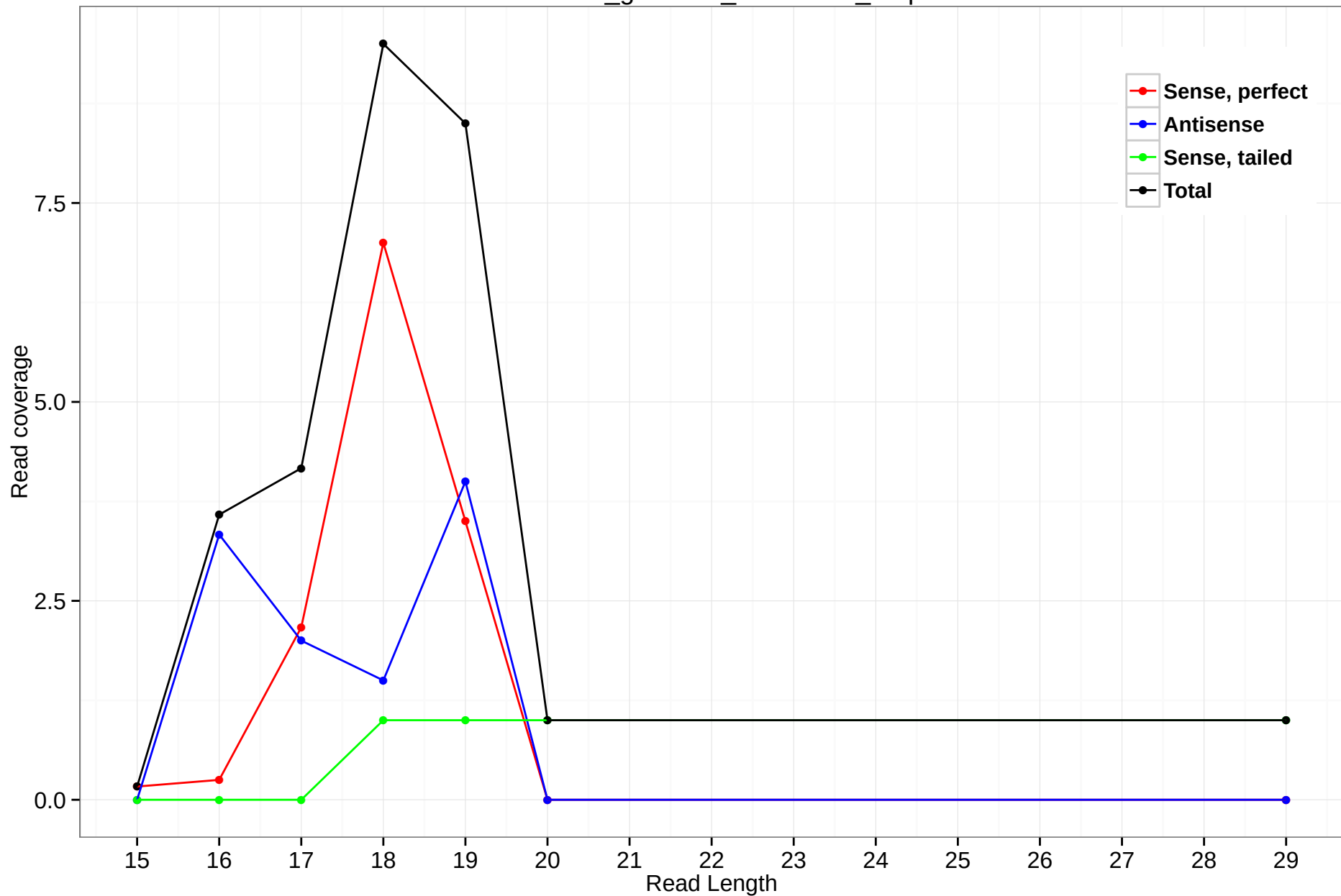
rheMac3_genscan_chr2.1740_1.3p
