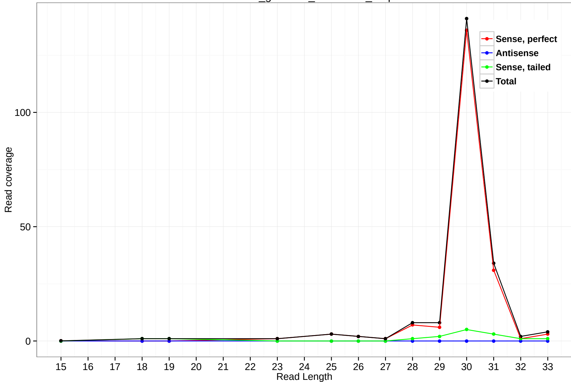
rheMac3_genscan_chr2.1707_2.5p
